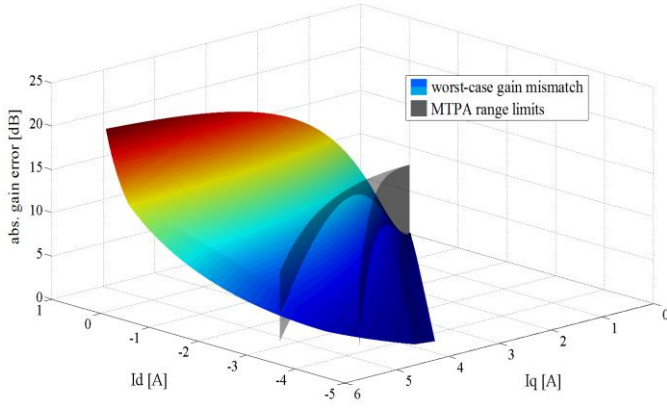
Fig. 7. Worst-case gain variation related to \pm 25\% parameters mismatch.
