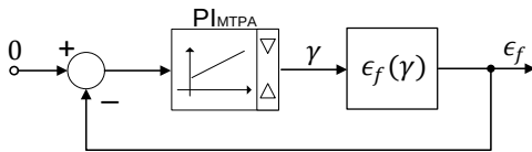
Fig. 5. Equivalent schematic for the tracking loop.
