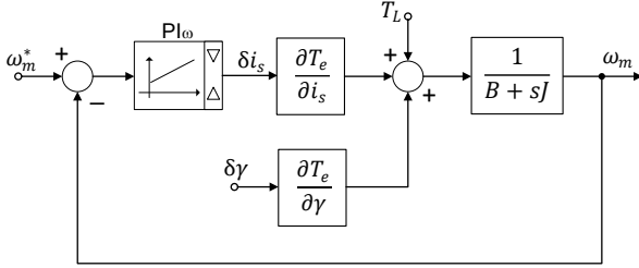
Fig. 4. Small-signal linearized equivalent model of the speed control loop.
