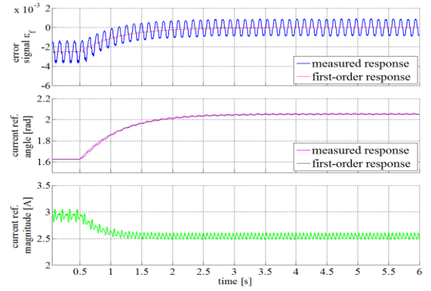
Fig. 12. MTPA tracking step response, all parameters as in Fig. 11 (top), except injection frequency is 25 Hz.
