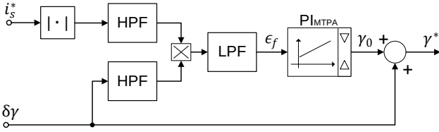
Fig. 3. MTPA tracking loop block diagram.
