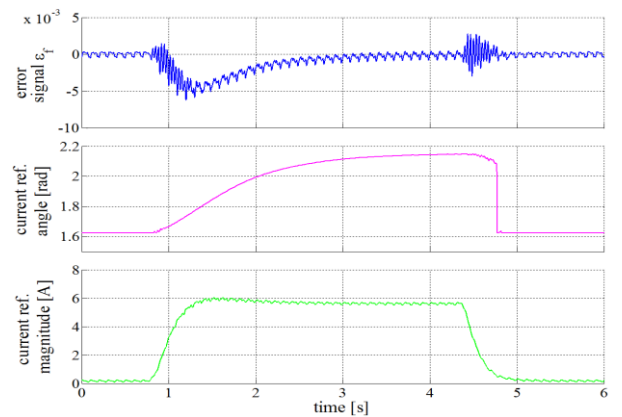
Fig. 15. MTPA tracking operation during 6 Nm load torque transient.
