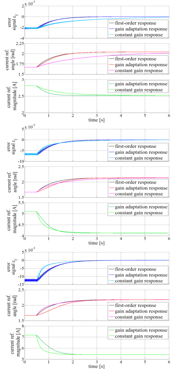
Fig. 8. MTPA tracking algorithm with and without gain adaptation: simulated step response test at 500rpm, load torque is 2, 4 and 6 Nm (from top to bottom respectively), injected signal is 50 mrad at 20 Hz.
