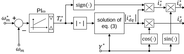
Fig. 2. Control scheme adopting torque reference and arbitrary current angle. applied to any control scheme implementing closed-loop MTPA tracking, e.g. [9][11][13].
