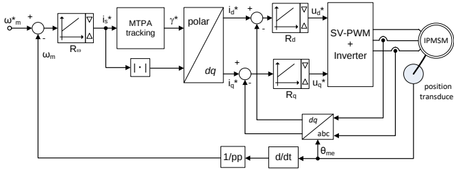
Fig. 1. Speed regulation with MTPA tracking implementation.
