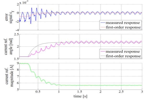
Fig. 13. MTPA tracking step response, test conditions as in Fig. 11 (bottom), injected signal is 12.5 mrad at 25 Hz, design tracking bandwidth is 1 Hz.
