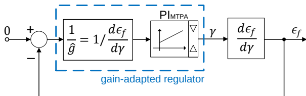
Fig. 6. Equivalent linearized schematic for the derivative-based normalization.
