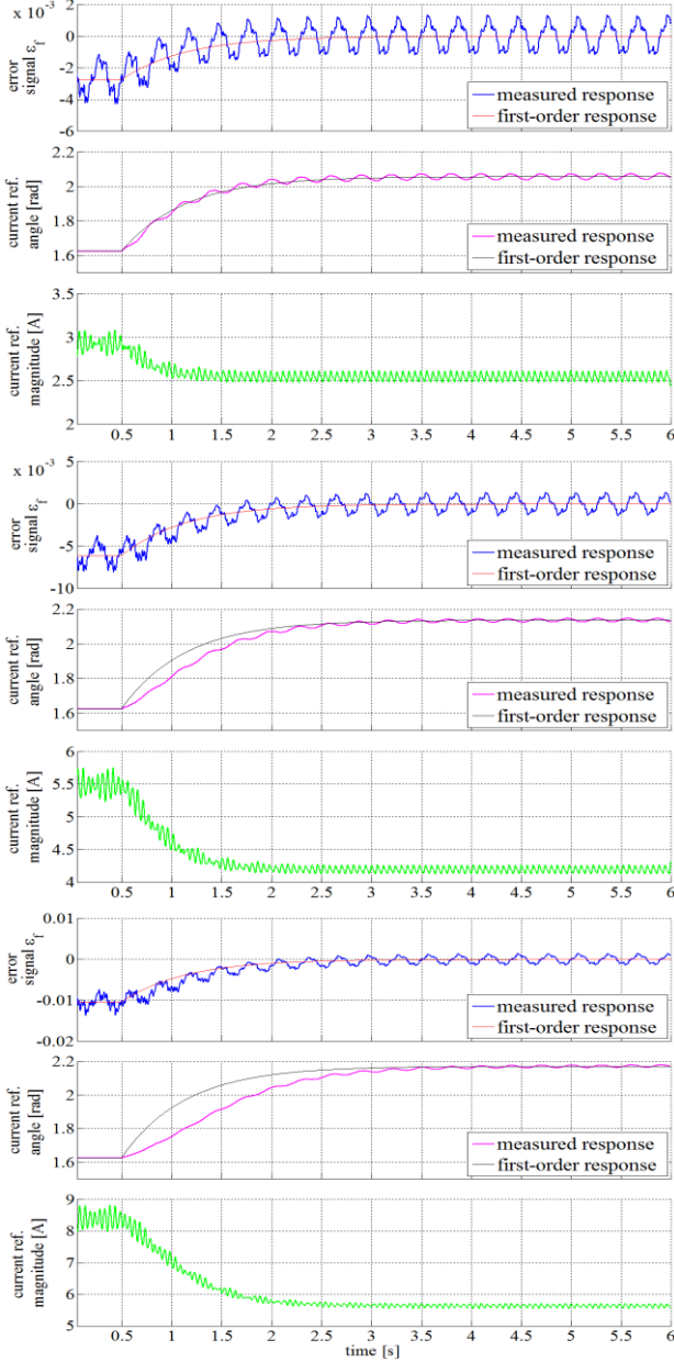
Fig. 11. Proposed MTPA tracking algorithm (0.25 Hz bandwidth): experimental step response test at 500rpm, load torque is 2, 4 and 6 Nm (from top to bottom respectively), injected signal is 50 mrad at 20 Hz.
