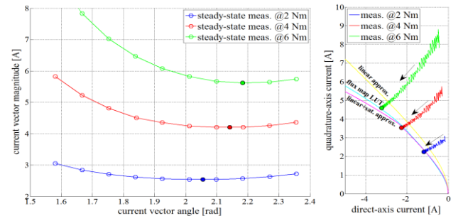
Fig. 14. Steady-state current space vector magnitude vs. angle under different load values (left) and dynamical trajectories in the dq current plane (right).
