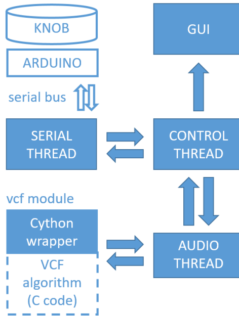
Figure 4.9: Python software architecture for interactive control of an audio effect with the haptic knob.
