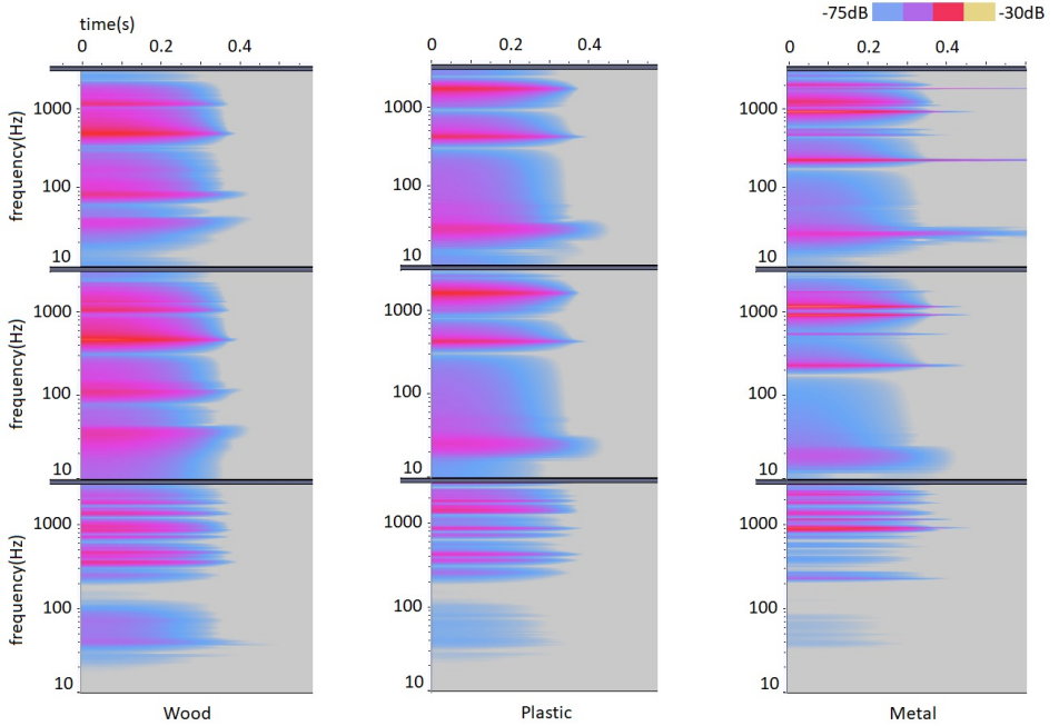
Figure 1.5: Vibration spectrograms in Experiment 1 (top row) and 2 (middle row). Vibrations reproduced on the glass plate in Experiment 2 (bottom row).
