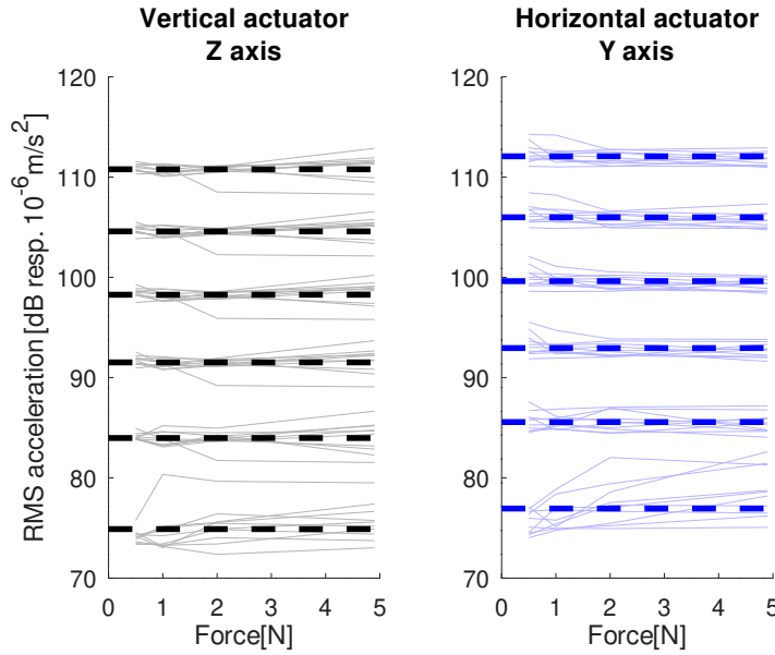
Figure 3.5: Acceleration measurements for all subjects (solid lines) and models (dashed lines) for the main direction of motion: Z axis for the vertical actuator (left plot) and Y axis for the horizontal actuator (right plot).
