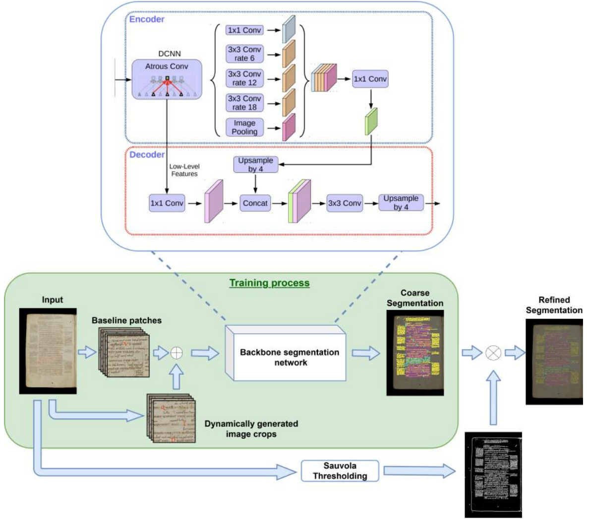
Fig. 2: Visual representation of the segmentation pipeline for the proposed framework. The green area represents the processes carried out during the training phase, where each input image is split into 2 sets of patches: the baseline patches, which are non-overlapping patches of size k \times k providing a complete representation of the original image and a set of C random crops which are extracted from random locations of the image at each training epoch. These 2 sets of patches are then combined and given in input to the backbone segmentation model which provides a predicted coarse segmentation map for each of them. These maps are compared with the ground truth ones through the application of a weighted cross-entropy loss. At inference time the dynamic instance generation step is removed while a segmentation refinement process is applied to the outputs of the backbone architecture to obtain more precise segmentation maps
