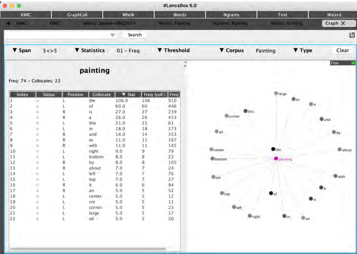
Figure 15 Strongest collocations of the word 'Painting'.
