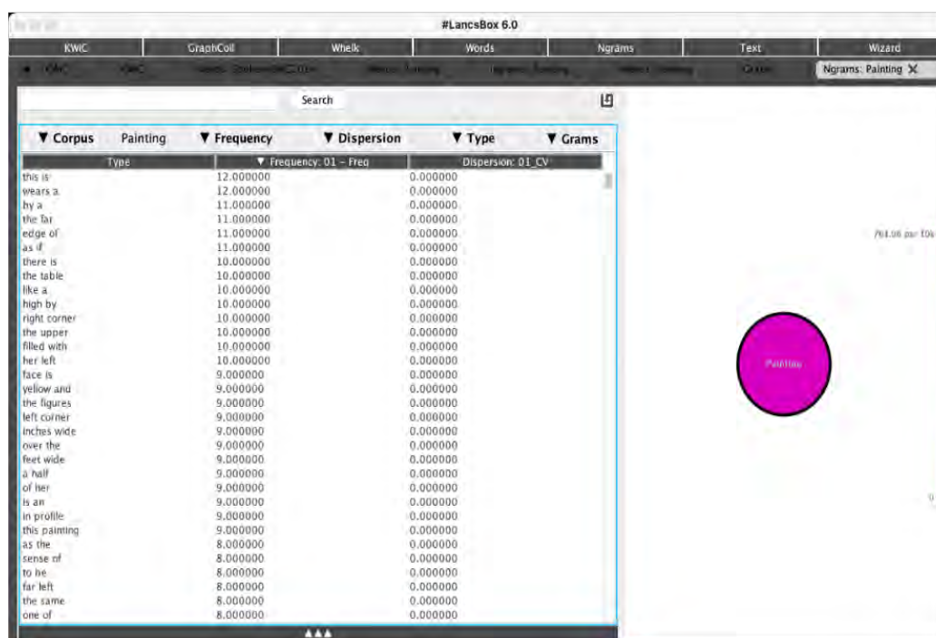
Figure 16 Most frequent N-Grams in the Painting corpus.
