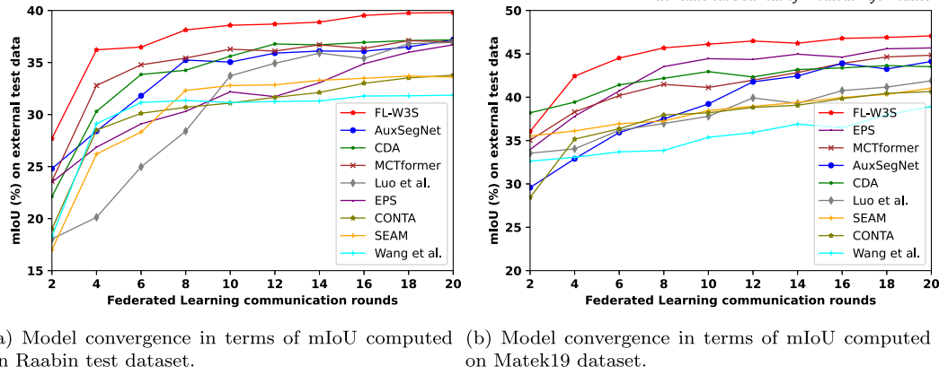
Fig. 4. Model convergence for the comparison of proposed FL-W3S method with the existing methods in terms of mean IoU (%) vs FL communication rounds.
