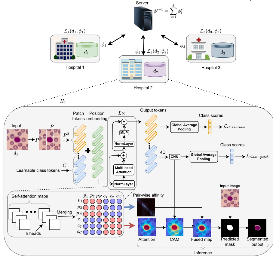
Fig. 1. FL-W3S architecture: A multi-class token transformer model training on cross-domain FL scenario produces class-specific attention maps. Pair-wise affinity obtained from patch-to-patch transformer attention is used to refine the object localization map. (For interpretation of the color(s) in the figure(s), the reader is referred to the web version of this article.)
