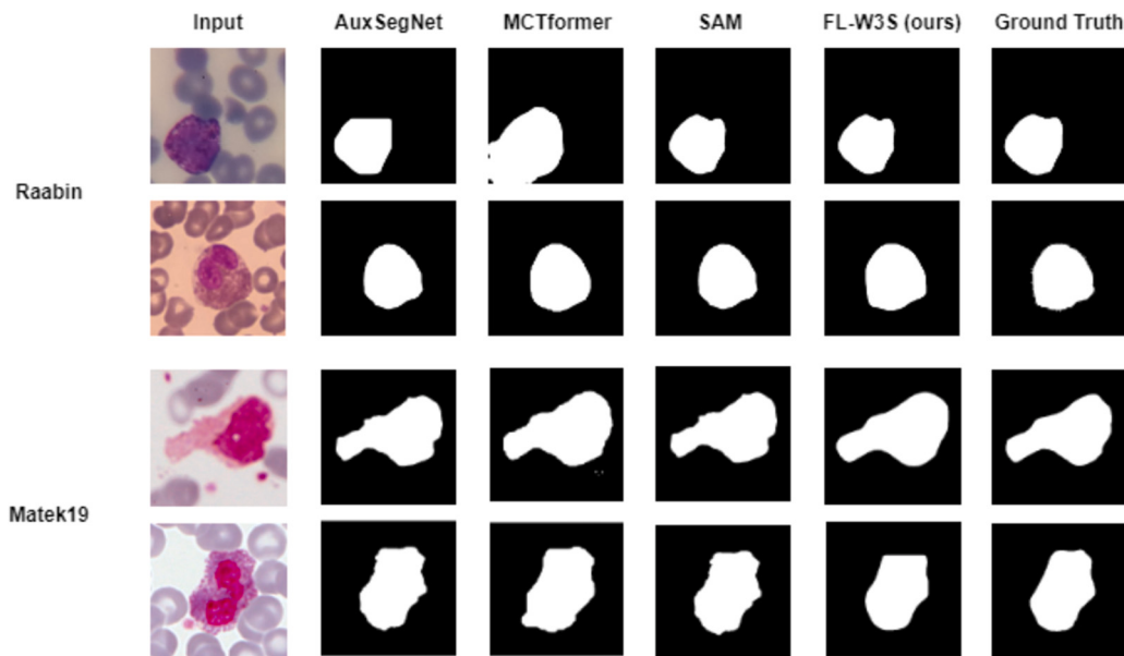
Fig. 3. Visual comparison of the proposed model with existing methods. Two random input images and their ground truth masks for each dataset (i.e., Raabin and Matek19) are selected for the comparison of the proposed method with existing competitive methods.
