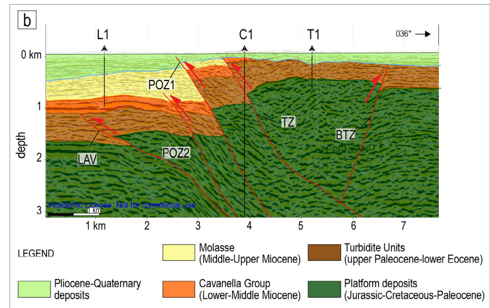
Fig. 27 - A) shaded relief map of the Pozzuolo del Friuli area (orange line: section trace of Fig. 27B), B) geological cross-section, derived from the conversion of interpreted ENI seismic line, across the Pozzuolo terrace showing the structure of the Pozzuolo Thrust System. Acronyms: BTZ: Terenzano Backthrust; LAV: Lavariano Thrust; PA: Panzano Thrust; POZ1 and 2: Pozzuolo1 and 2 Thrusts; TV: Trivignano Thrust; TZ: Terenzano Thrust; UB: Udine-Buttrio Thrust. C1: Cargnacco; L1: Lavariano; T1: Terenzano exploration wells.
