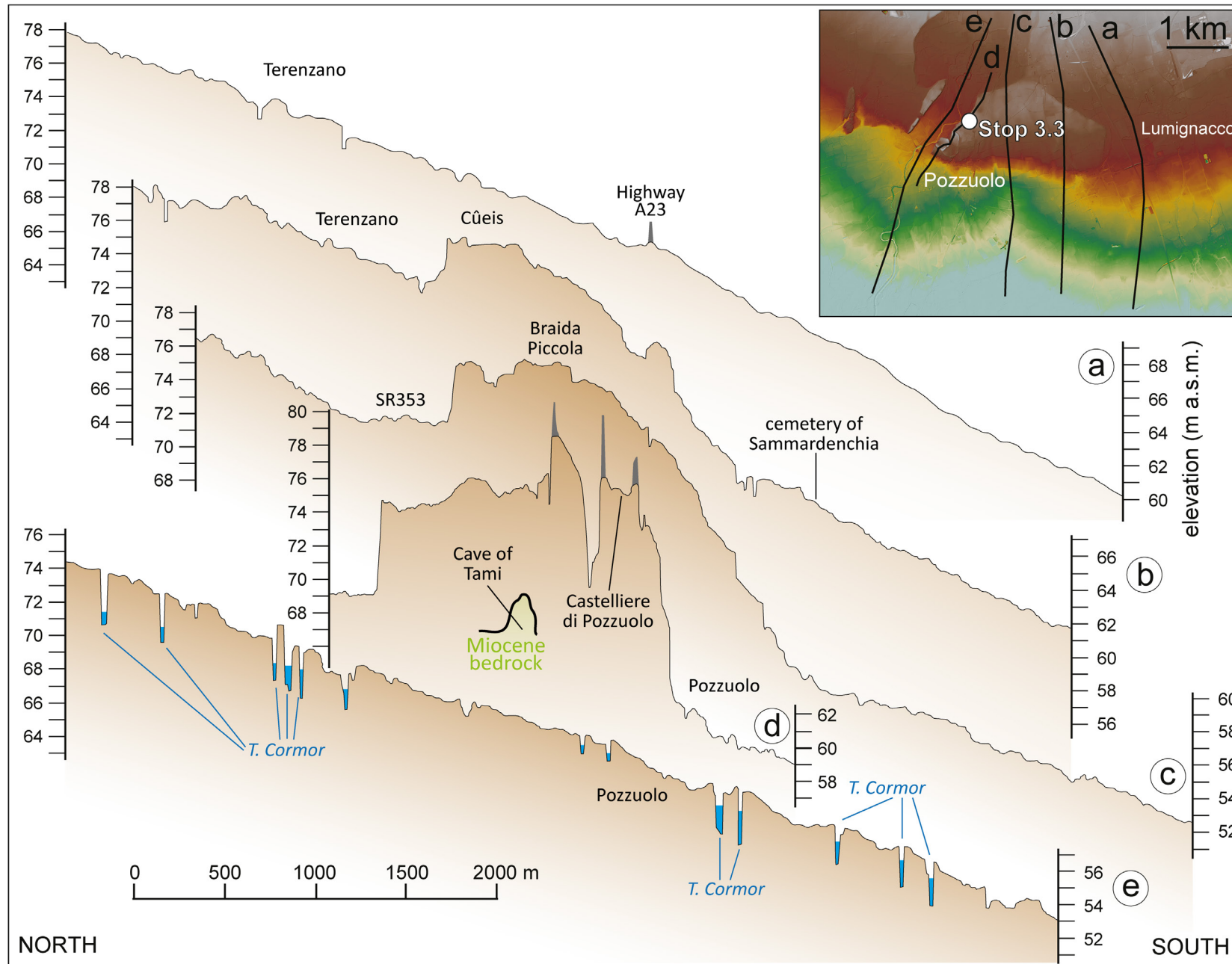
Fig. 29 - Topographic profiles perpendicular to the slope of the plain (Fontana and Ferrari, 2020). For the location, see the black traces indicated in the inset map at the top right.
