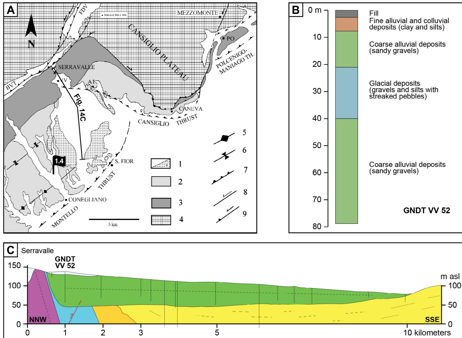
Fig. 14 - A) Geological sketch map of the Vittorio Veneto area (Stop 1.4). Legend: 1) Quaternary deposits; 1a) moraines of the Vittorio Veneto glacial tongue; 2) Conegliano complex (clays, sands, conglomerates; Middle-Pliocene – Lower Pleistocene); 3) Southalpine Molasse (upper Oligocene-Miocene); 4) carbonate successions (Jurassic-Cretaceous), Scaglia Rossa Fm. (Upper Cretaceous - lower Eocene), marly-arenaceous flysch (Eocene); 5) anticline; 6) syncline; 7) thrust; 8) strike-slip fault; 9) transpressive fault; A1: Anzano 1 well; BVT: Bassano-Vittorio Veneto thrust; PO: Polcenigo, FDV: Fadalto valley. B) Simplified lithological log of GNDT_VV52 borehole near Serravalle. C) Cross section of the Vittorio Veneto Basin (trace in Figure 14A); the hypothetical trend of the buried “geological” bedrock is derived from borehole stratigraphies (marked VV). Pre-Quaternary bedrock: violet: lower Cavanella group and Monte Baldo fm. (Lower-Middle Miocene); blue: Tarzo marl (Serravallian); orange: Vittorio Veneto sandstone and Montello conglomerate (Tortonian-Messinian); yellow: Conegliano complex (Pliocene - Lower Pleistocene); green: gravelly or sandy-gravelly body; grey: clay, silt and sand (Middle Pleistocene – Holocene). Note that in the SSE end of the profile, the Miocene bedrock rises up because of Montello thrust activity. Heavy dark lines indicate the water table (mod. after Avigliano et al., 2008).
