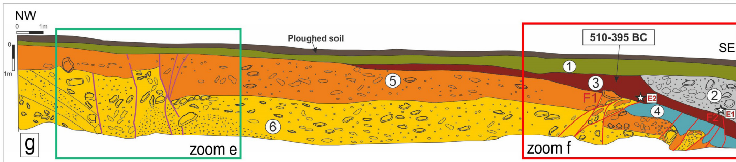
Fig. 23 - A) Palaeoseismological trench MEDUNO_EAST; B) the shear zone affected the southern edge of the trench; C) particular of the shear zone affected the historical unit 3; D) interpretation of MEDUNO-EAST trench wall. Red lines: reverse faults. E) extrados fractures at the northern portion of the trench MEDUNO-WEST (green rectangle); F) damage zone localised near the tectonic scarp of trench MEDUNO-WEST (red rectangle); G) interpretation of MEDUNO-WEST trench wall. One metre for the mesh grid. Numbers refer to stratigraphic units; E1 and E2: identified seismic events; F1 and F2: fault planes (mod. after Poli et al., 2021a).
