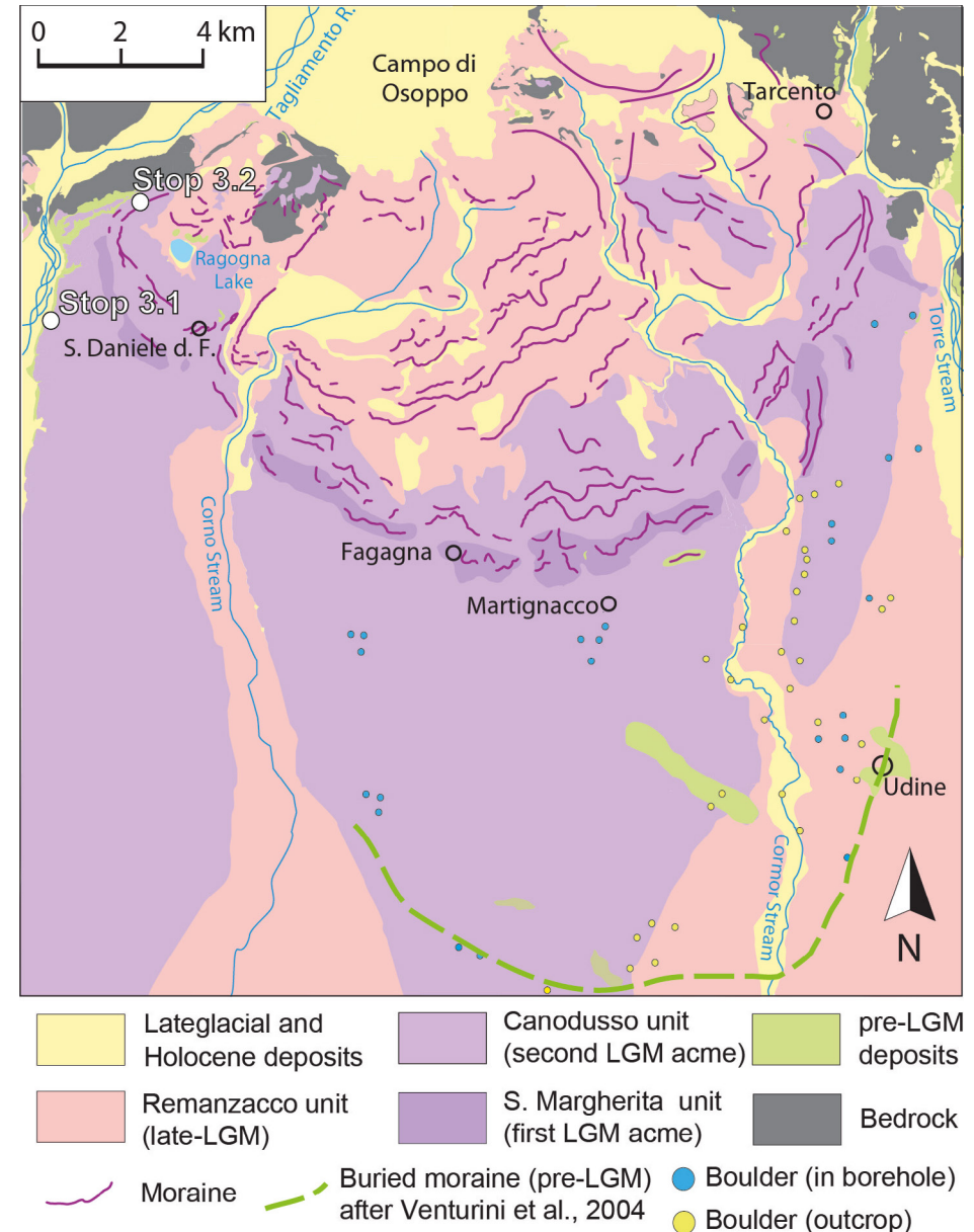
Fig. 26 - Geological map of the Tagliamento end moraine system and the related outwash plain (mod. after Monegato et al., 2020).
