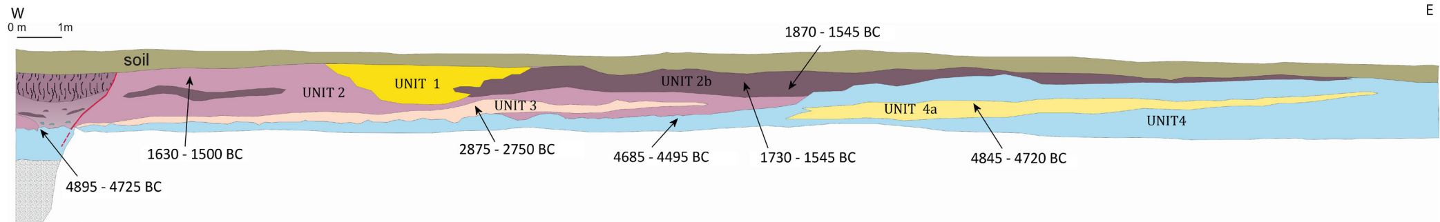
Fig. 17 - Geognostic trench in the NE portion of Palù di Livenza basin (Stop 2.1, see Fig 15 for location). Unit 1: anthropogenic filling; Unit 2 and 2b: clayey-silty peaty sediments with sand lenses (Unit 3); Unit 4: lacustrine deposits, with bioturbations (4a) to the left, the paleo-liquefactions. Northern wall of the trench.
