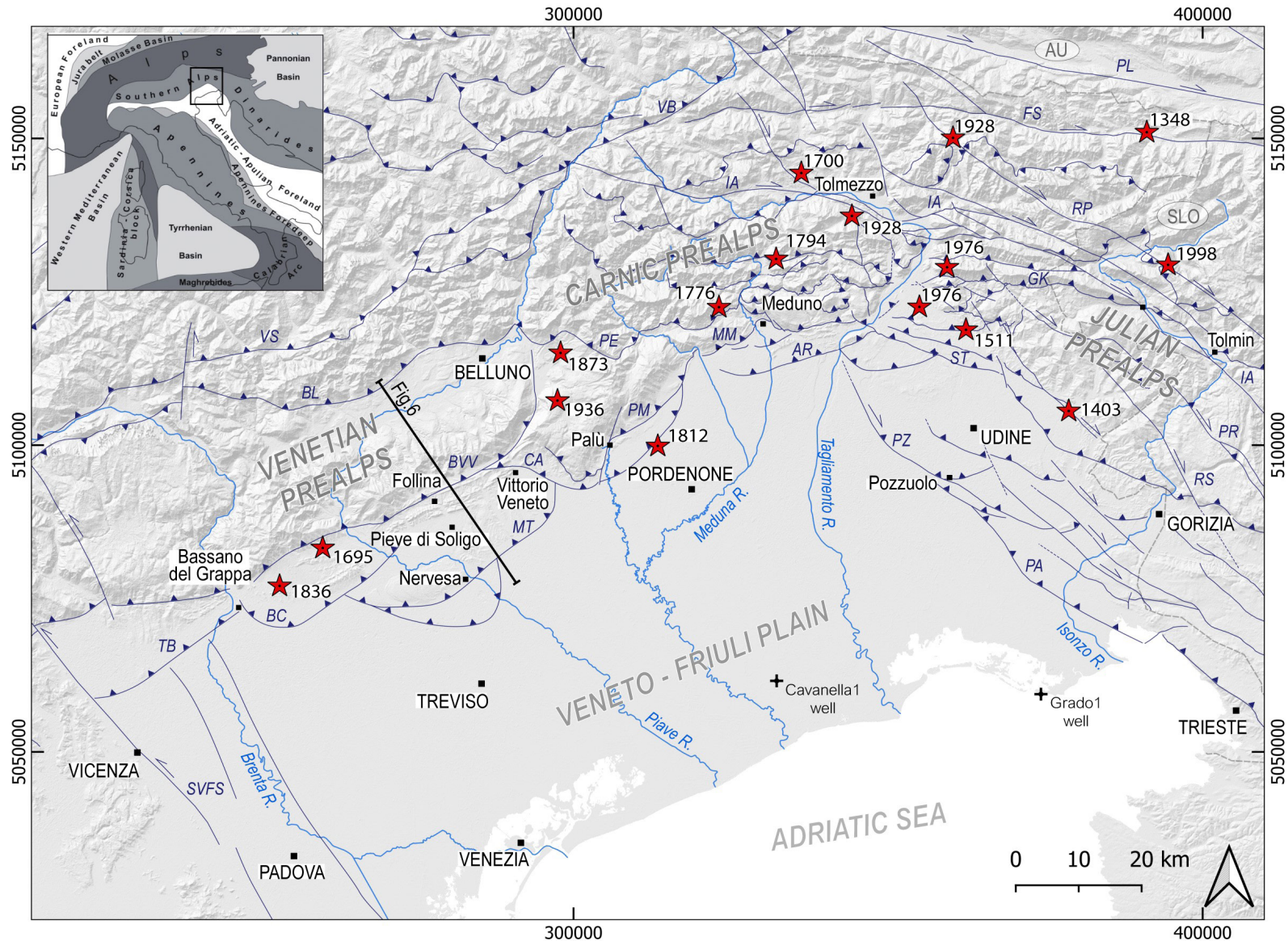
Fig. 2 - Structural sketch map of the eastern Southern Alps in NE-Italy and W-Slovenia. Red stars: historical and instrumental seismicity ( M_w > 5.5 ; Rovida et al., 2022). Legend: AR: Arba-Ragogna Thrust; BC: Bassano-Cornuda Th.; BL: Belluno Th.; BVV: Bassano–Vittorio Veneto Th.; CA: Cansiglio Th.; FS: Fella–Sava Fault; GK: Gemona–Kobarid Th.; IA: Idrija–Ampezzo Fault; MM: Meduno-Maniago Th.; MT: Montello Th.; PA: Palmanova Th.; PE: Periadriatic Th.; PL: Periadriatic Lineament; PM: Polcenigo-Montereale Th.; PR: Predjama Fault; PZ: Pozzuolo Th.; RP: Ravne–Paularo Fault; RS: Raša Fault; ST: Susans-Tricesimo Th.; SVFS: Schio-Vicenza Fault System; TB: Thiene-Bassano Th.; VSVB: Valsugana-Val Bordaglia Th.
