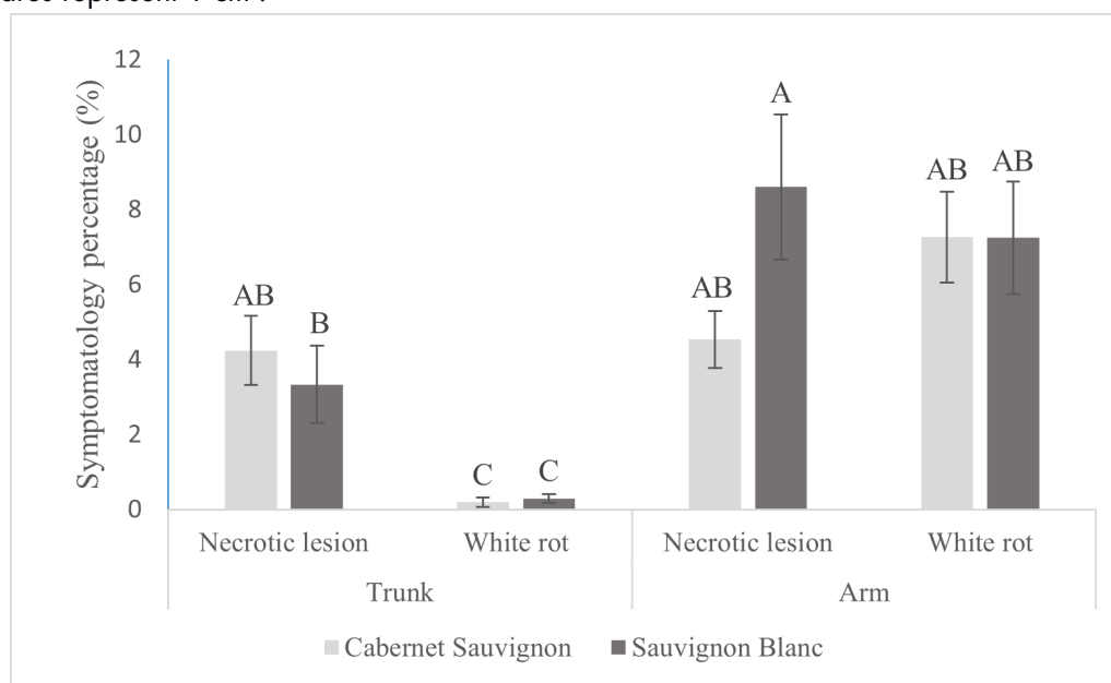
FIGURE 2. Percentage of symptomatic area (mm 2 ) ± standard error in trunks and arms of Cabernet-Sauvignon (CS) and Sauvignon blanc (SB) for necrotic lesion and white rot symptoms. Different letters indicate significant differences (Tukey post hoc test, p \leq 0.05 ).
