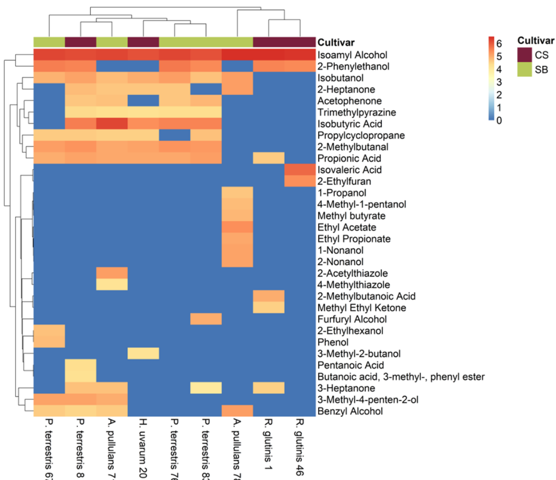
FIGURE 6. Heatmap of VOC profiles across yeast strains with hierarchical clustering values corresponding to the log10-transformed peak areas. Colour intensity reflects the relative abundance of each compound.
