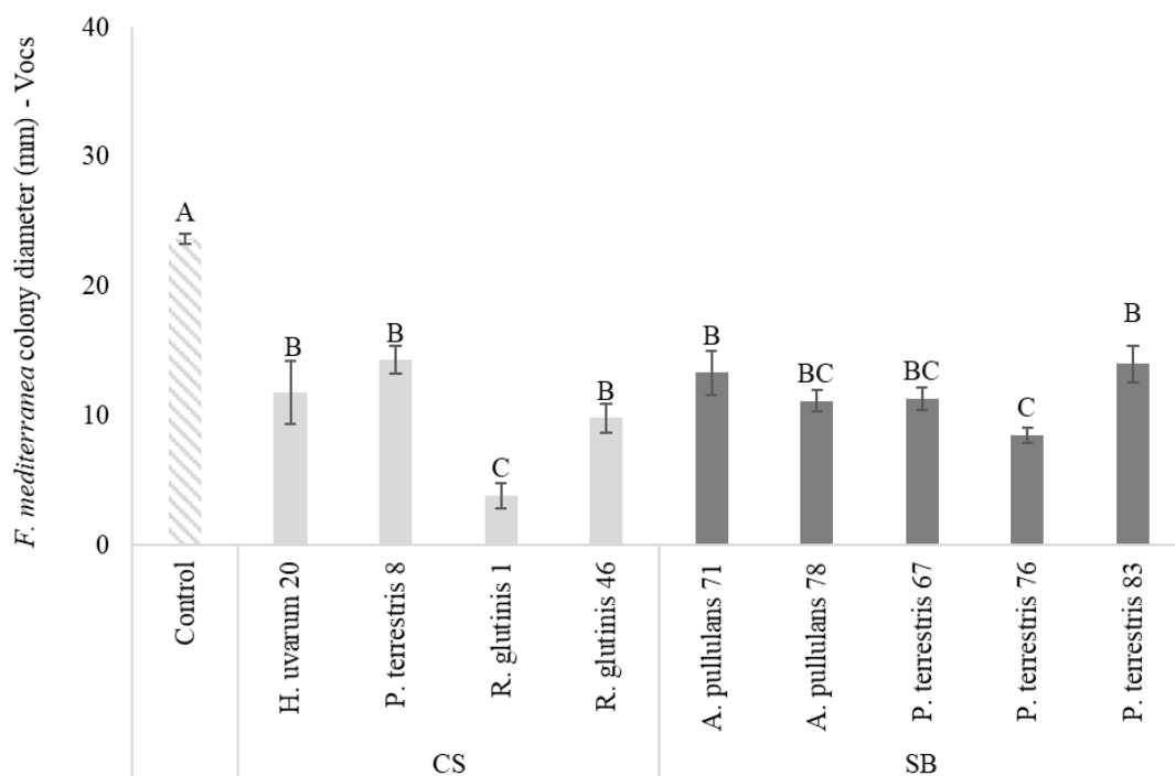
FIGURE 5. Fomitiporia mediterranea colony diameter (mm ± standard deviation) when exposed to the VOCs produced by the yeasts isolated from Cabernet-Sauvignon (CS) and Sauvignon blanc (SB) grapevines. Different letters indicate statistically significant differences within each grapevine cultivar group (Tukey post hoc test, p \leq 0.05 ).
