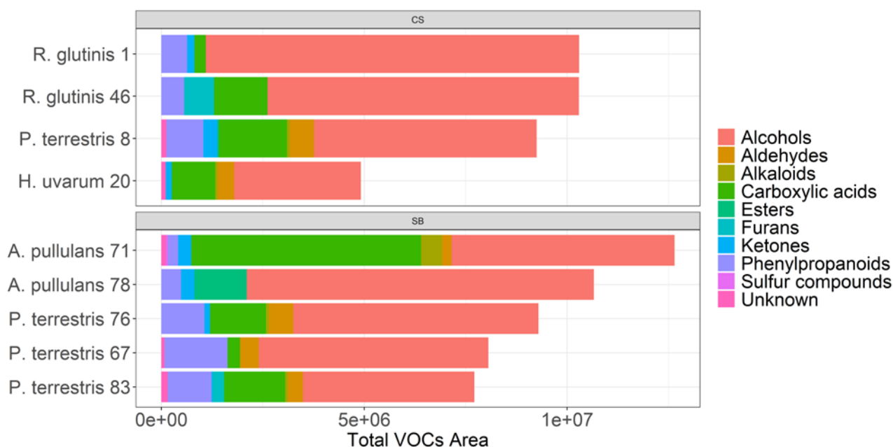
FIGURE 7. Composition of yeast strains' volatilome. Bars represent the absolute area of detected VOCs for each examined yeast strain. Different colours indicate different compounds' chemical classes. Yeast strains are grouped by grapevine cultivar (Cabernet-Sauvignon, CS; Sauvignon blanc, SB).
