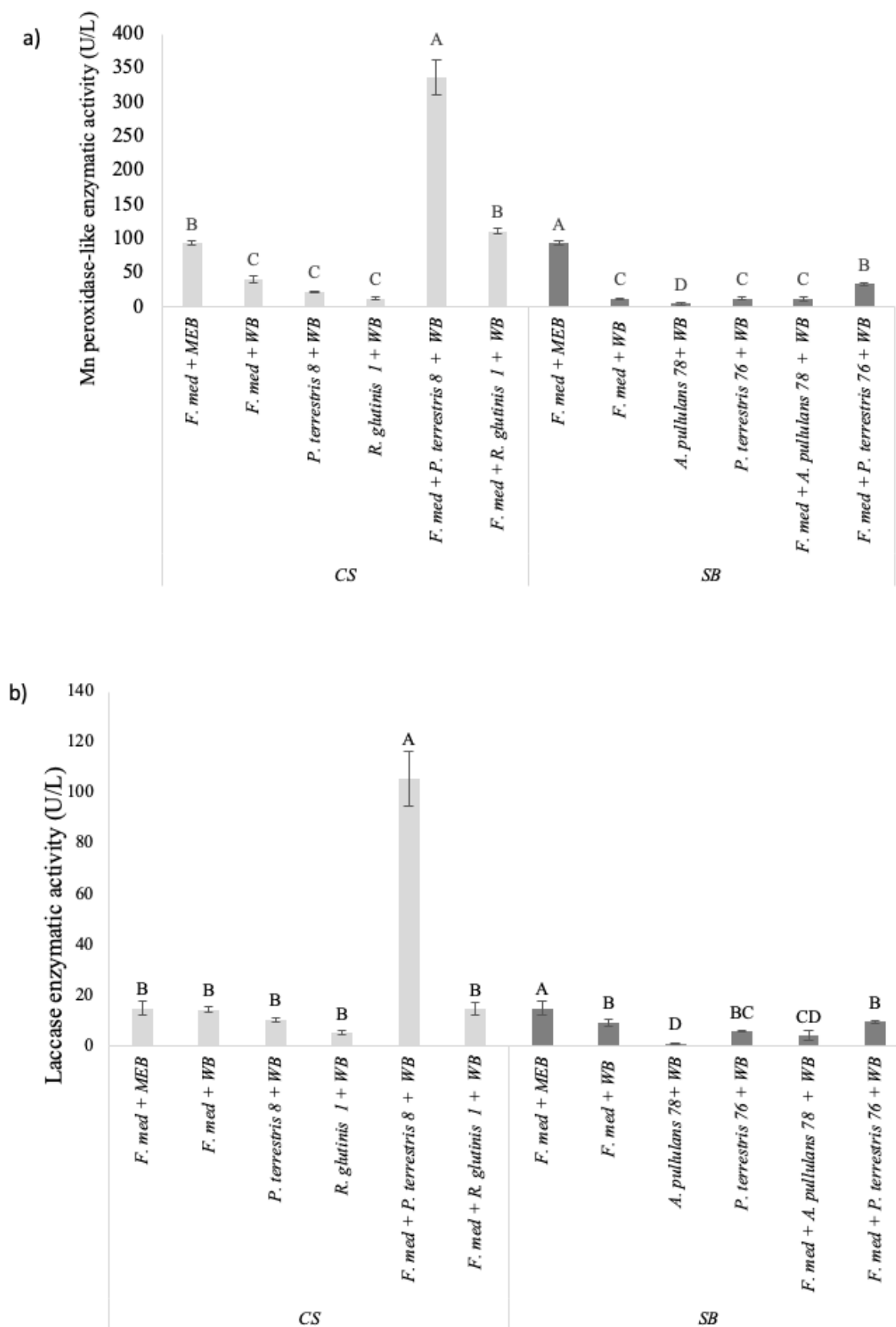
FIGURE 8. Mn peroxidase-like (a) and laccase-like (b) activity (U/L) \pm standard deviation of Fomitiporia mediterranea ( F. med ) and endophytic yeasts grown in different media (MEB: Malt Extract Broth; WB: Wood Broth), alone or in co-culture. Different letters indicate statistically significant differences within each grapevine cultivar group (Cabernet-Sauvignon, CS; Sauvignon blanc, SB) (Tukey post hoc test, p \leq 0.05 ).
