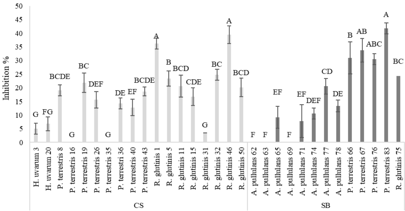
FIGURE 3. Inhibition percentage of Fomitiporia mediterranea mycelial colony growth (% ± standard deviation) by the yeasts isolated from Cabernet-Sauvignon (CS) and Sauvignon blanc (SB) grapevines, in the dual culture assay. Different letters indicate significant differences within each grapevine cultivar group (Tukey post hoc test, p \leq 0.05 ).
