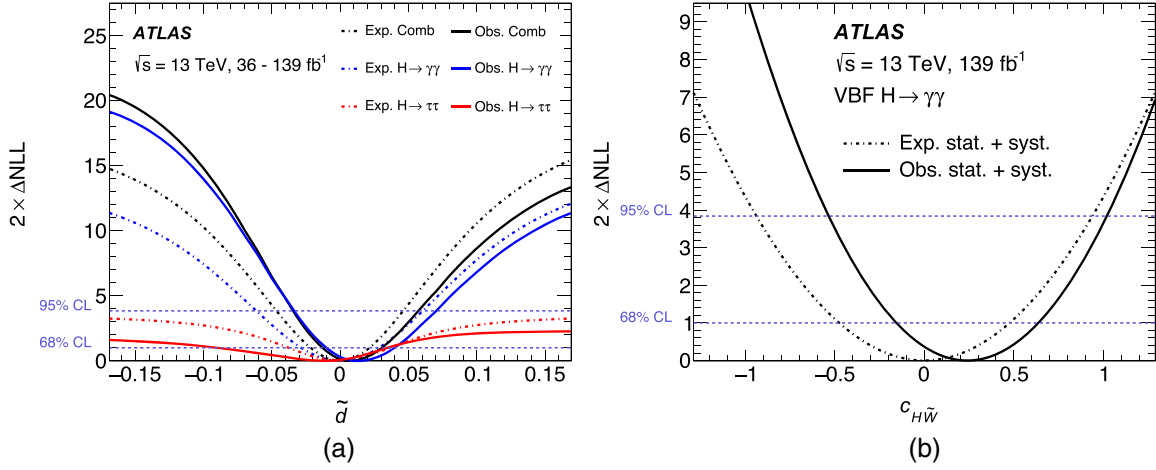
FIG. 3. \Delta\text{NLL} curves as a function of (a) \tilde{d} and (b) c_{H\bar{W}} . In (a), the \Delta\text{NLL} of \tilde{d} considers the interference-plus-quadratic terms, whereas in (b) the \Delta\text{NLL} of c_{H\bar{W}} considers the interference-only term. The solid lines are the observed results, while the dashed lines are the expected results. In (a), the blue lines represent the results of this analysis, while the red lines represent the results from the H \rightarrow \tau\tau analysis [9]. The black lines show the combination of these two analyses. For all figures, the dashed horizontal lines show the values of \Delta\text{NLL} used to define the 68% and 95% confidence intervals.
