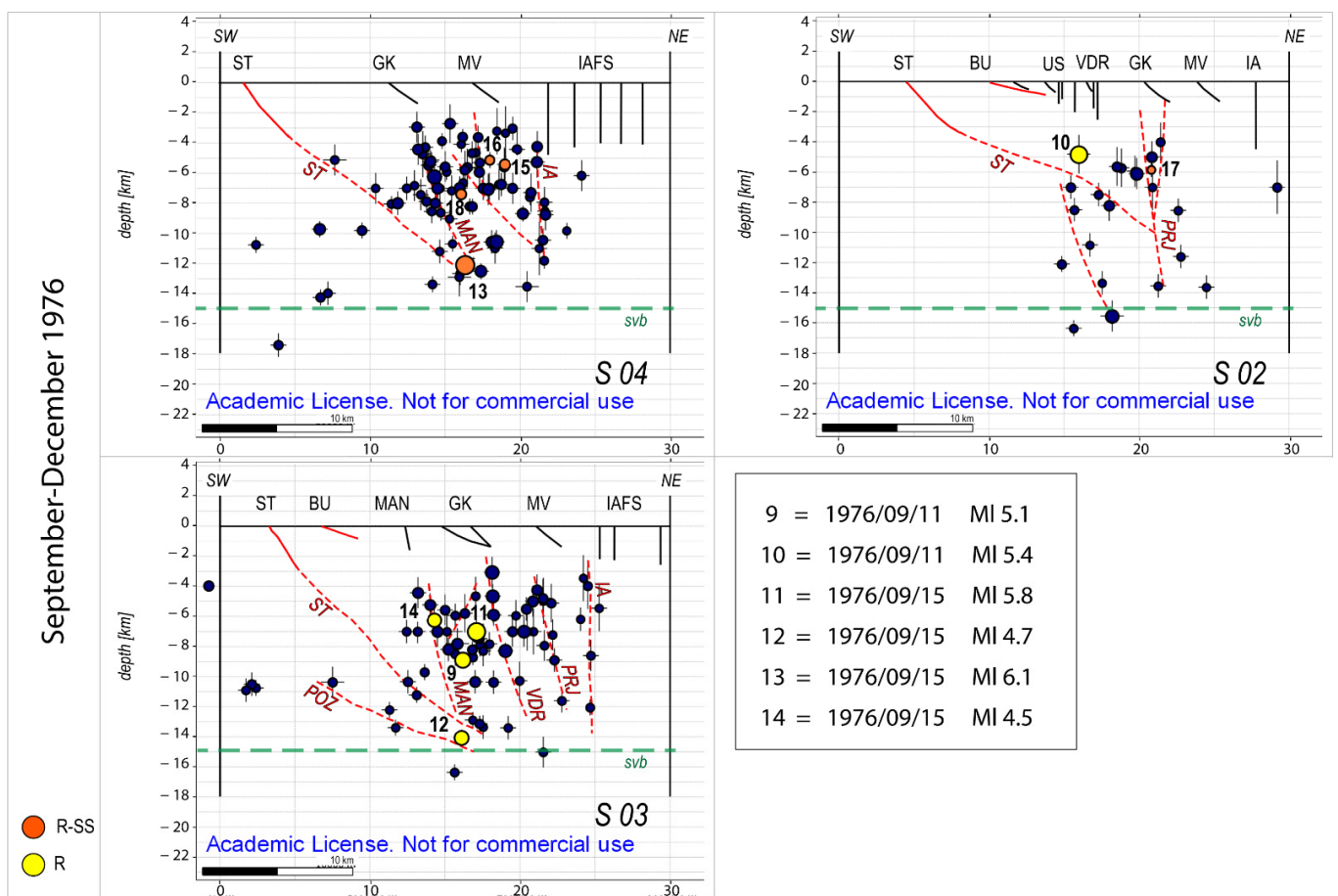
Figure 9. September–December 1976 Ml \geq 2.5 seismicity (dark blue circles) plotted on the seriated sections 01–04 (see traces in Figure 6) together with the active faults’ surfaces reconstructed in this study (red thrusts) and tectonic structures known from the literature (black faults, [27]). The symbol’s size is proportional to the magnitude value (Ml), the number of the events refers to Table 2, while the color refers to the kinematics as shown in the legend. The vertical and horizontal bars for each event represent the vertical (Z) and horizontal (H) error localization, respectively. The red dashed lines refer to the interpretations of the activated structures, recognized on each section. The green dashed line represents the base of the seismogenic volume (svb). Fault acronyms: BFC: Borgo Faris–Cividale Fault System; BU: Buia Thrust; GK: Gemonà–Kobarid Th.; IAFS: Idrija–Ampezzo Ft. System; MV: Musi–Verzegnis Th.; PRJ: Predjama Ft.; ST: Susans–Tricesimo Th.; VDR: Vedronza Fault; US: Useunt Ft.
