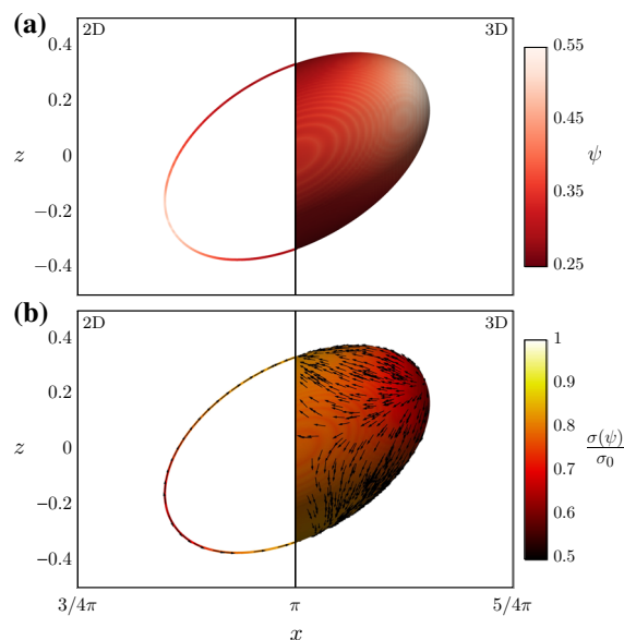
Fig. 8 Panel a shows the surfactant distribution over the droplet interface. Due to the action of the external shear stress, surfactant accumulates at the droplet front and back, while the droplet belly is depleted of surfactant. Panel b depicts the dimensionless surface tension, \sigma(\psi)/\sigma_0 , over the droplet interface. The Marangoni stresses, which originate from the surface tension gradients, are reported using black unit length vectors. In both panels, results obtained from 2D cases are reported on the left while those obtained from 3D cases are reported on the right. The snapshots are taken at t = 2.5 (steady-state deformation) and refers to the case H3 ( \psi_b = 0.02 , Ca = 0.187 )
