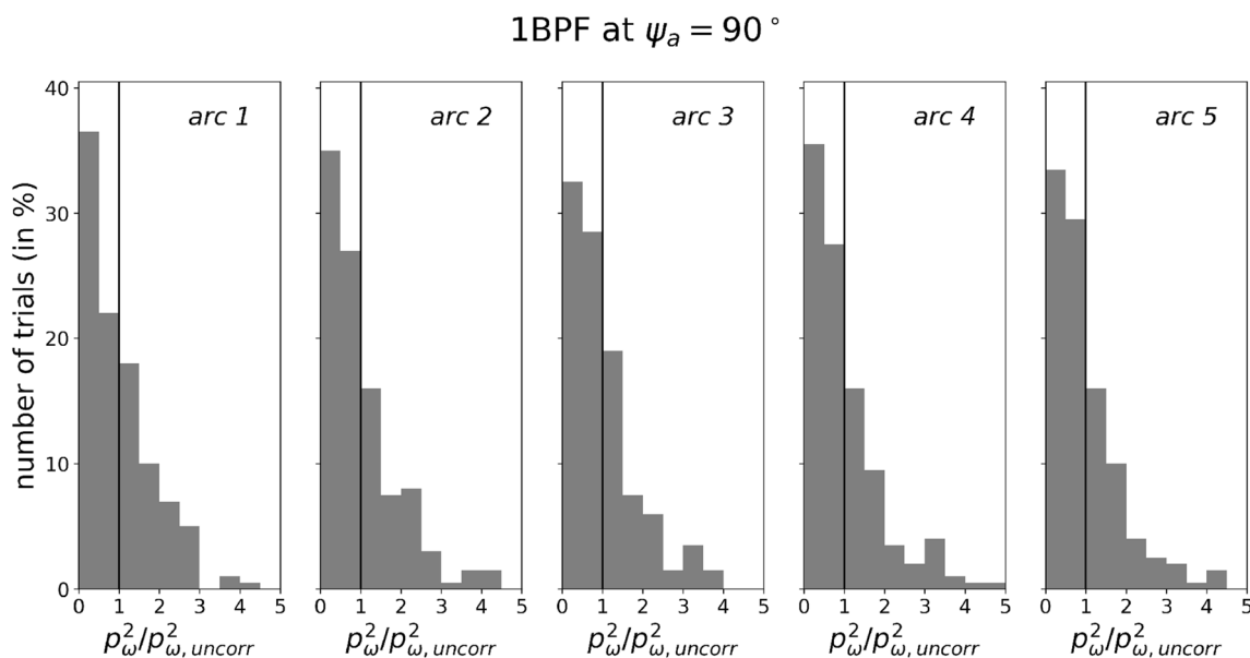
Fig. 22 Probability distribution of p_{\omega}^2 |_{\Sigma_{corr}} for the 200 trials
