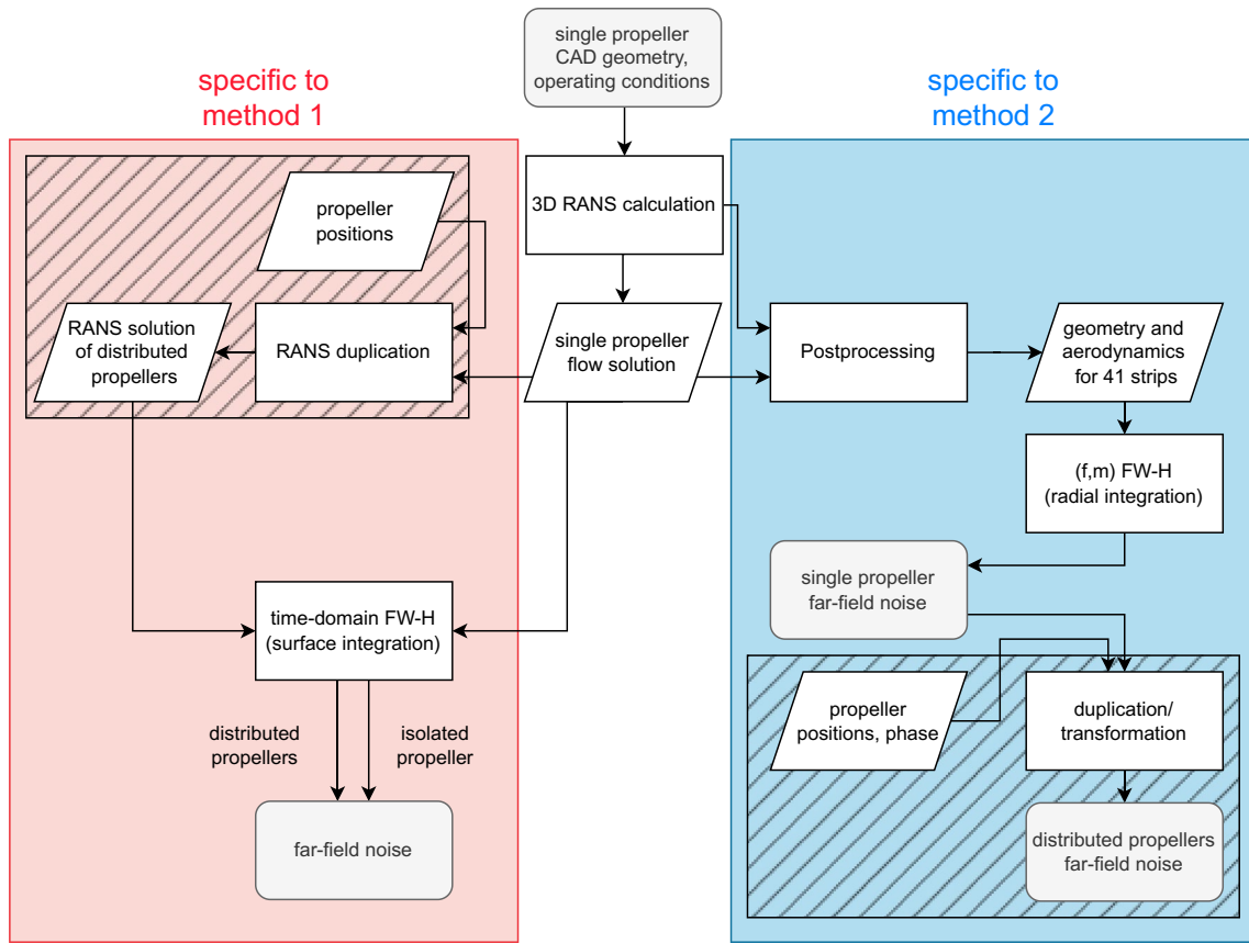
Fig. 1 Workflow of both methods applied in this work; the dashed areas encompass the tasks specific to the multi-propeller configuration
