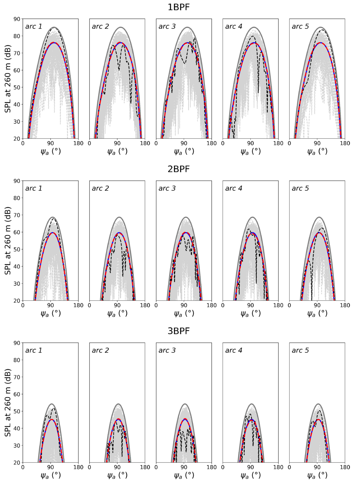
Fig. 21 Probability analysis: results on the sound directivity: (light gray solid lines) all 200 directivities, (red dashed lines) mean directivity, (blue solid lines) directivity assuming uncorrelated propellers,
