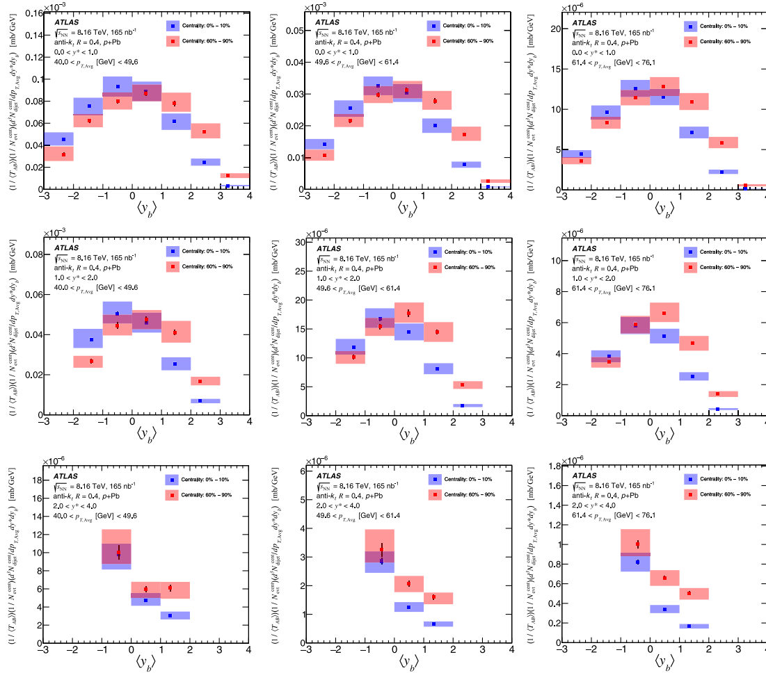
FIG. 4. \langle T_{AB} \rangle normalized per-event dijet yields in 0%–10% (blue) and 60%–90% (red) collisions as a function of \langle y_b \rangle in three representative p_{T, \text{Avg}} bins for 0.0 < y^* < 1.0 (top row), 1.0 < y^* < 2.0 (middle row), and 2.0 < y^* < 4.0 (bottom row). Shaded rectangles represent the total systematic uncertainty, while the vertical error bars represent the statistical uncertainty. The systematic uncertainties for the two distributions are highly correlated.
