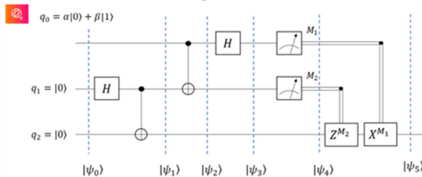
Figure A1. Examples from the specific path “Quantum computing”. Screenshots of the slides used during the lecture. Top : single-qubit gates. Left middle : two-qubit gates. Left bottom : teleportation protocol. Right-bottom : one step of the mathematical description of the quantum random walk protocol.
