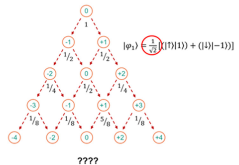
Figure A1. Examples from the specific path “Quantum computing”. Screenshots of the slides used during the lecture. Top : single-qubit gates. Left middle : two-qubit gates. Left bottom : teleportation protocol. Right-bottom : one step of the mathematical description of the quantum random walk protocol.
