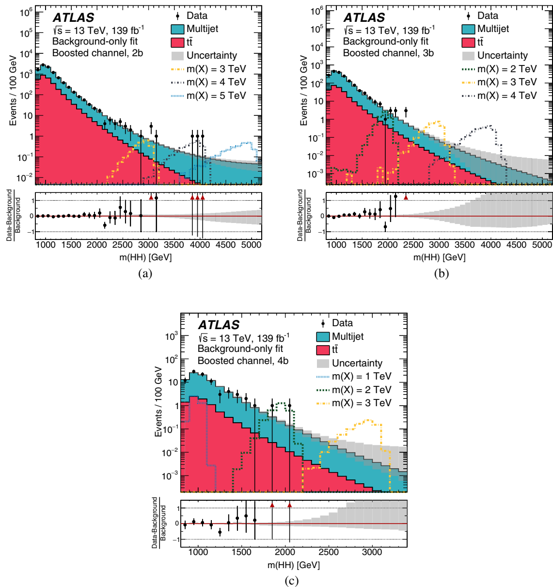
FIG. 13. The m(HH) distributions in the boosted (a) 2b , (b) 3b , and (c) 4b signal regions (dots), after the fit under the background-only hypothesis. The error bars on the data points represent the Poisson uncertainties corresponding to their event yields. The background model (stacked histogram) is shown with its total post-fit uncertainty (gray band). The uncertainty bands are defined using an ensemble of curves constructed by sampling a multivariate Gaussian probability density function built from the covariance matrix of the fit. Representative spin-0 signal hypotheses (dashed and dashed-dotted lines) are overlaid, normalized to the overall expected limits on their cross sections. The bottom panel shows the difference between the data and the background model, normalized to the background model. No significant excess of data relative to the SM background is observed.
