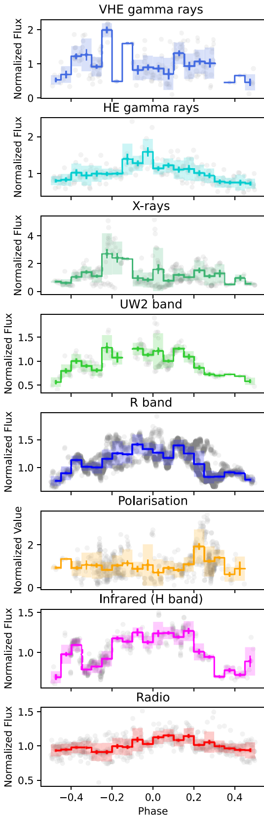
Figure 9. PG 1553 + 113 MWL folded light curves obtained by assuming a period of 798 d. In each panel, the average values are reported with a continuous line. The error bar in each bin is the standard error of the mean values. The coloured bar in each bin represents the variance of the data distribution.
