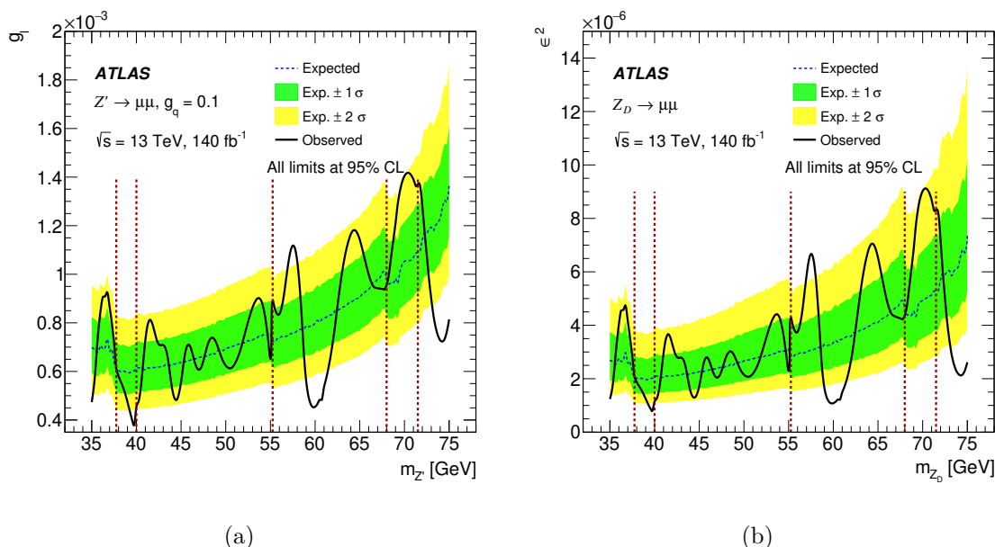
Figure 9. (a) Observed and expected 95% CL upper limits on the coupling between the Z' boson and leptons as a function of m_{Z'} , assuming g_q = 0.1 . (b) Observed and expected 95% CL upper limits on the kinetic mixing parameter ( \epsilon^2 in the dark photon model) as a function of m_{Z_D} . Discontinuities correspond to the boundaries between different GP hyper-parameter regions. Vertical dashed lines indicate the mass points where the hyper-parameters are changed.
