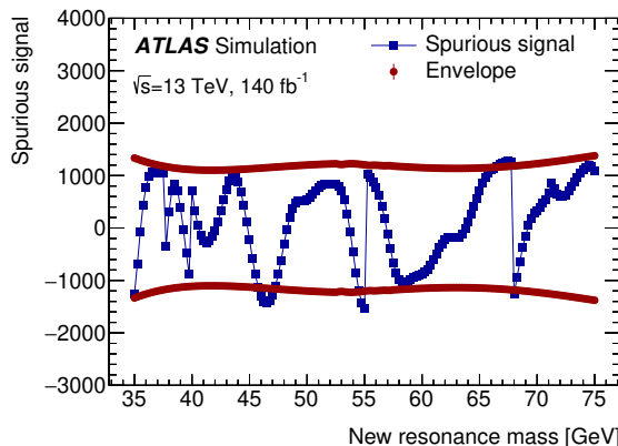
Figure 5. Spurious signal yield as a function of the new resonance mass, obtained by fitting signal-plus-background models to background-only templates. The points represent the fitted signal yields, with vertical error bars indicating the corresponding statistical uncertainties. The thick curves denote the symmetrised envelope, which defines the systematic uncertainty associated with the background modelling. Discontinuities in the spurious signal reflect transitions between different Gaussian process hyper-parameter configurations.
