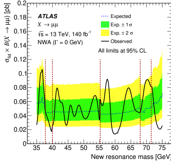
Figure 8. Observed and expected 95% CL upper limits on the production fiducial cross-section times branching ratio of a narrow-width ( \Gamma = 0 \text{ GeV} ) resonance, as a function of the new resonance mass. Discontinuities correspond to the boundaries between different GP hyper-parameter regions. The vertical dashed lines indicate the mass points where the hyper-parameters are changed.
