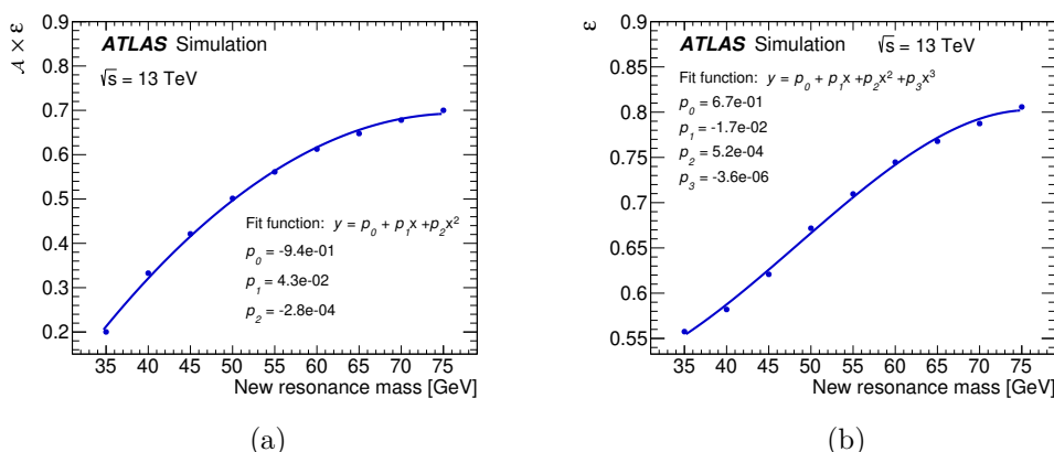
Figure 2. Parameterisation of the acceptance and efficiency for the new resonance. (a) The product of acceptance and efficiency ( \mathcal{A} \times \varepsilon ) as a function of the resonance mass, fitted with a second-order polynomial. (b) The detector correction factor (efficiency, \varepsilon ) as a function of the resonance mass, fitted with a third-order polynomial.
