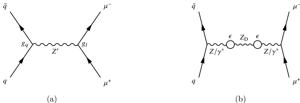
Figure 1. Feynman diagrams for Drell-Yan production of (a) a generic resonance Z' and (b) a kinetically mixed dark photon Z_D .
