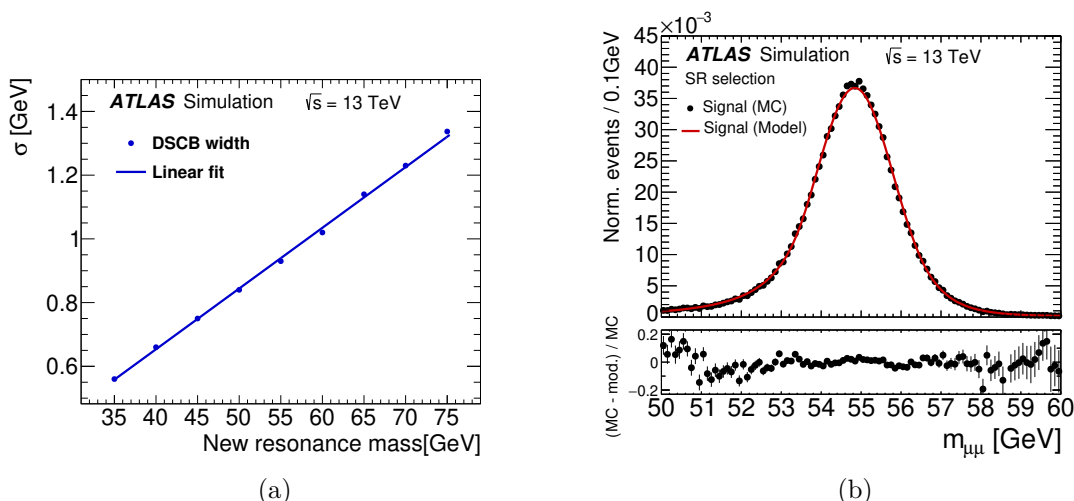
Figure 3. (a) Width of the DSCB Gaussian core as a function of the new resonance mass (solid markers), with a linear fit overlaid. (b) Simulated dimuon mass distribution for a hypothetical Z' resonance with a mass of 55 GeV and a width \Gamma = 0.21 GeV (solid markers), overlaid with the signal model, defined as a Breit-Wigner distribution convolved with a DSCB function and obtained from a parametric fit to the signal template. The lower panel displays the relative difference between the MC simulation and the signal model.
