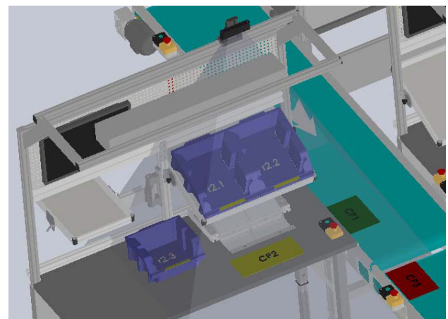
Fig. 4. Assembly table and control points.
