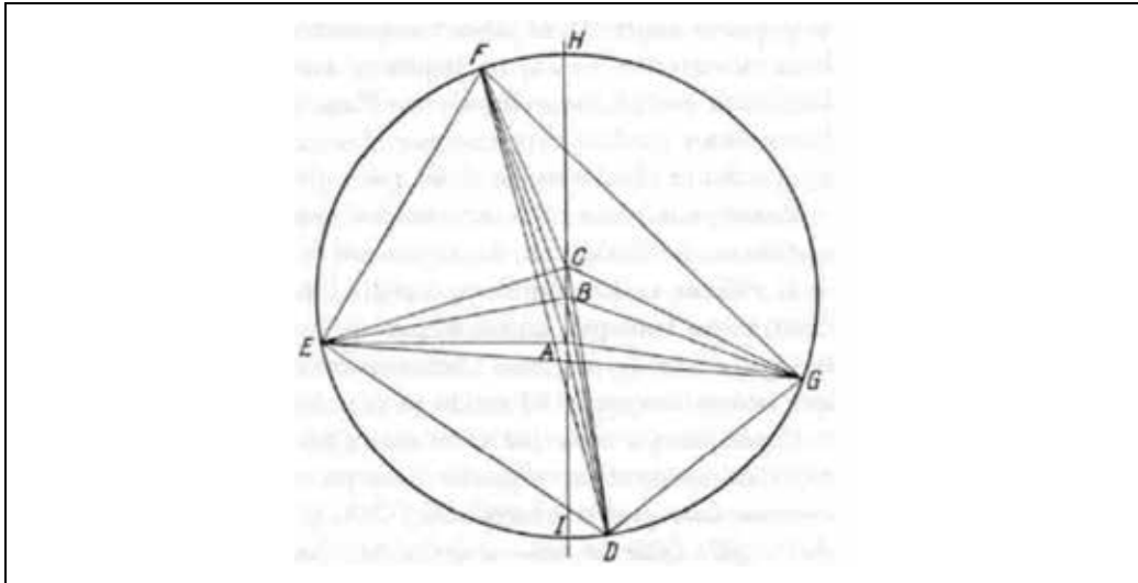
Fig. 1. The points D, G, F, E represent Mars' oppositions observed by Tycho respectively in 1587, 1591, 1593, 1595. Point A represents the Sun, point B the geometrical centre of the orbit and point C is the punctum aequans. The straight line HI is the line of apsides. Kepler obtained: a) the longitude of the aphelion (year 1587) that was 28^{\circ}48'55'' of the Lion constellation; b) posed equal to 1 the segment HD, the length of the segments BC=0,07232 and BA=0,11332 (KGW III, p. 153).
