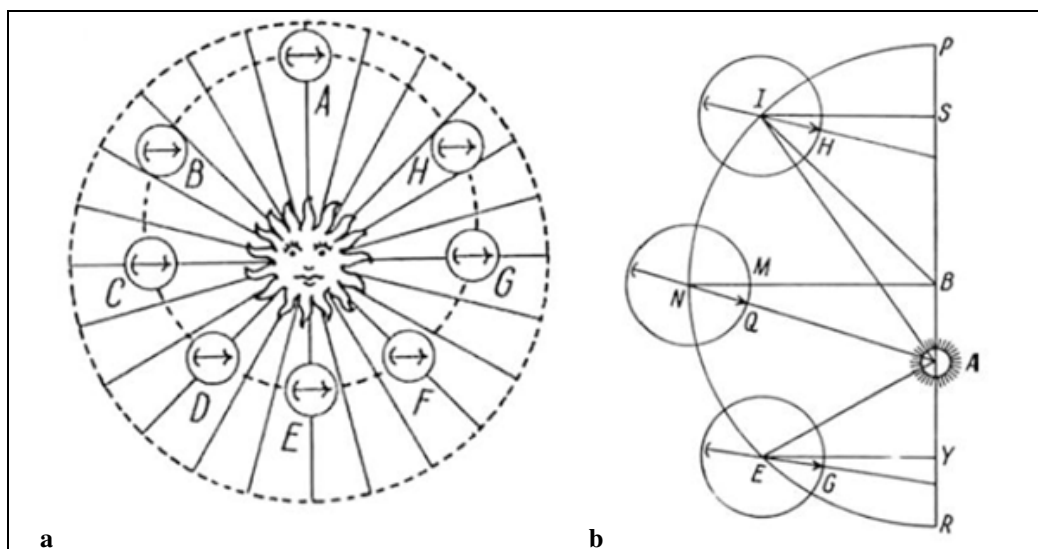
Fig. 2. a. General explanation of the force-mechanism determining the orbit’s ellipticity (Kepler 1618-1621, KGW VII, p. 337). b. When the centre of the Sun, the centre of the Planet and the amicus pole are aligned ( AQN ) the planet is in one of the two quadrature ( ibid. , p. 339)
