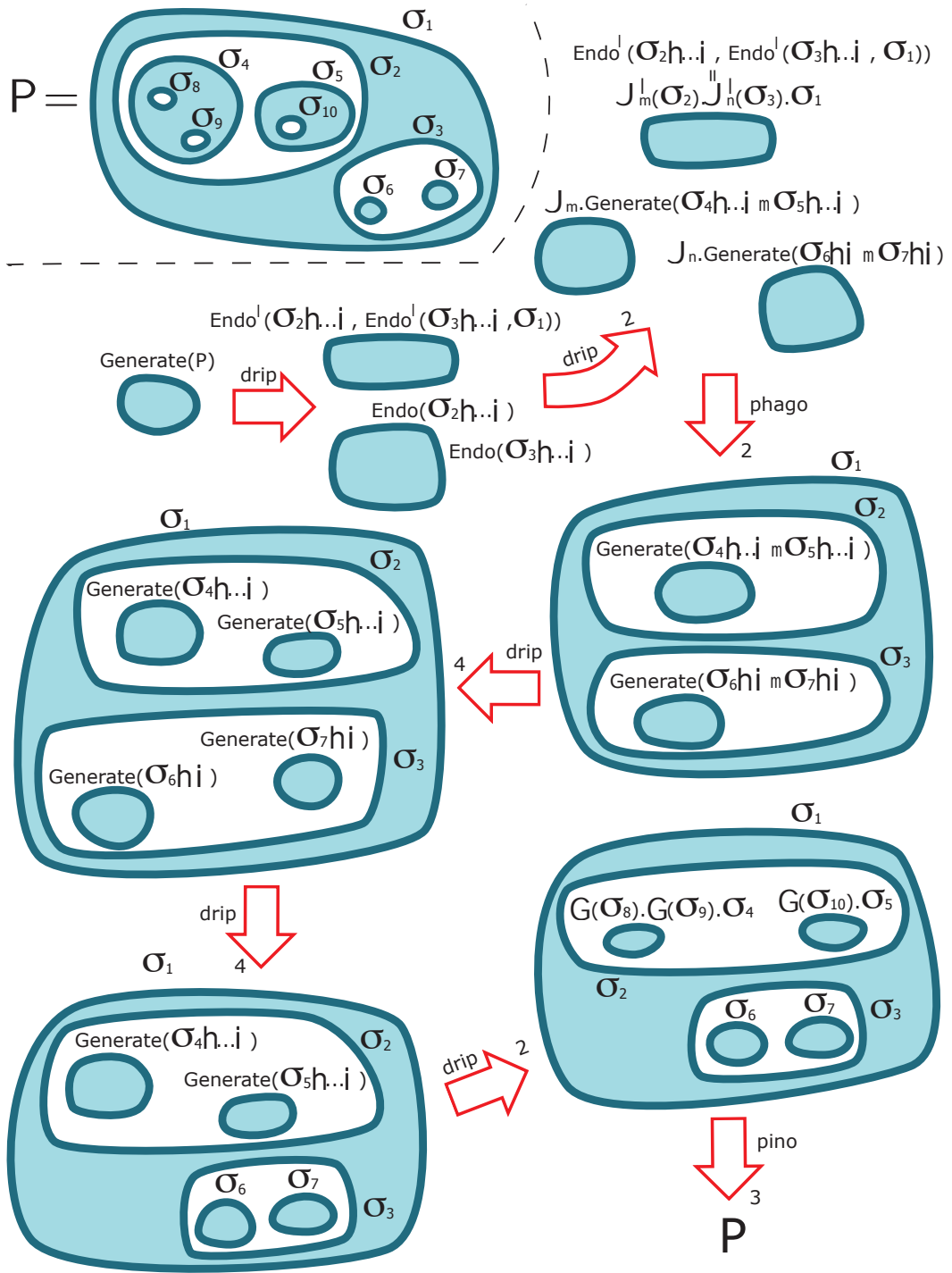
Fig. 1. \text{Generate}(P)(\diamond) reduces to P ( m, n are names not in \text{FN}(P) )
