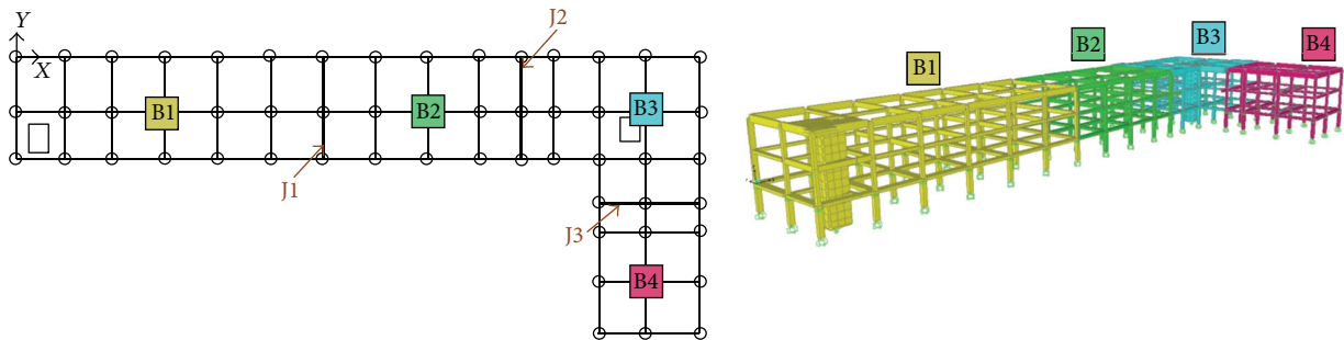
FIGURE 2: Numbering of the blocks (B1–B4) constituting the multiple building and relevant separation joints (J1–J3).
