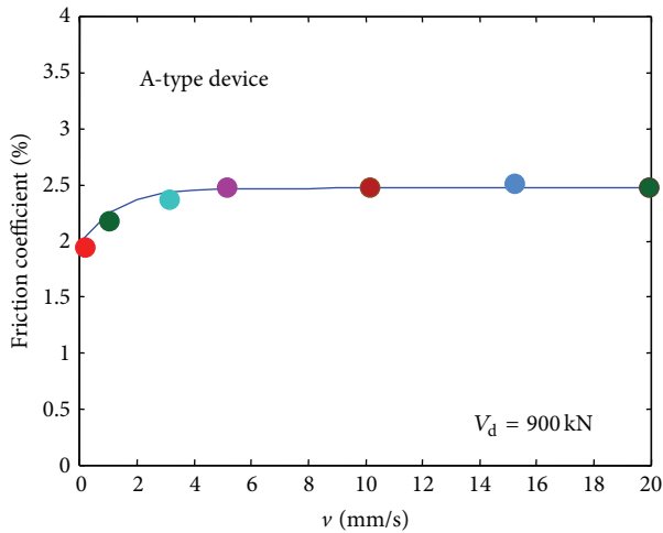
FIGURE 9: Friction coefficient values as a function of v —A-type isolator, V_d = 900 kN.
