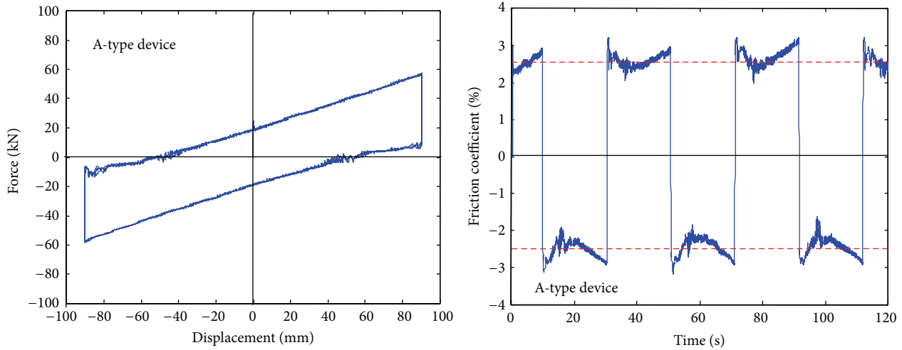
FIGURE 7: Response cycles and portion of the friction coefficient time-history obtained from a dynamic test carried out on one A-type isolator, with d_{c,max} = \pm 91 mm, v = 10 mm/s, and V_d = 900 kN.
