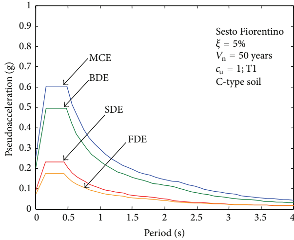
FIGURE 4: Normative pseudoacceleration elastic response spectra for Sesto Fiorentino—FDE, SDE, BDE, and MCE levels, \xi = 5\% , V_n = 50 years, c_u = 1 , topographic category T1, and C-type soil.
