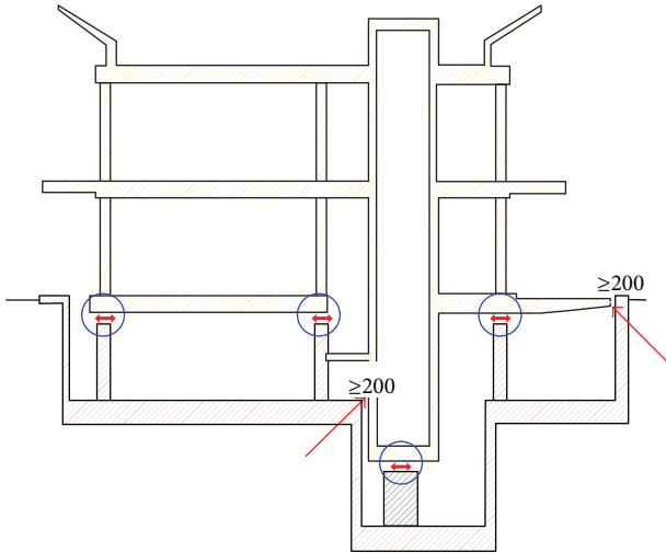
FIGURE 3: Schematic cross section in correspondence with the left elevator pit alignment, with isolators highlighted with circles and separation gaps between mobile and fixed structures with arrows.
