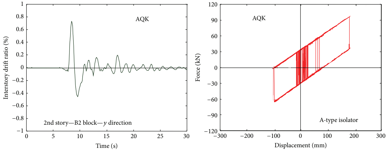
FIGURE 12: Second interstory drift ratio time-histories for B2 block and response cycles of most stressed DFP isolator obtained in y direction from the NS AQK input accelerogram.
