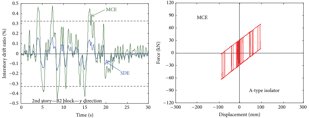
FIGURE 10: Second interstory drift ratio time-histories for B2 block and response cycles of most stressed DFP isolator obtained in y direction from the most demanding MCE-scaled input accelerogram.
