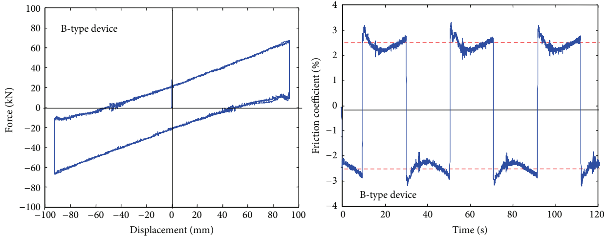
FIGURE 8: Response cycles and portion of the friction coefficient time-history obtained from a dynamic test carried out on one B-type isolator, with d_{c,max} = \pm 91 mm, v = 10 mm/s, and V_d = 1100 kN.
