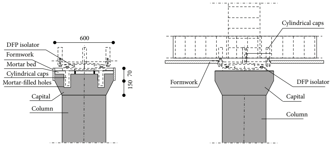
FIGURE 13: Design drawings concerning the installation details of a DFP isolator over a column.
