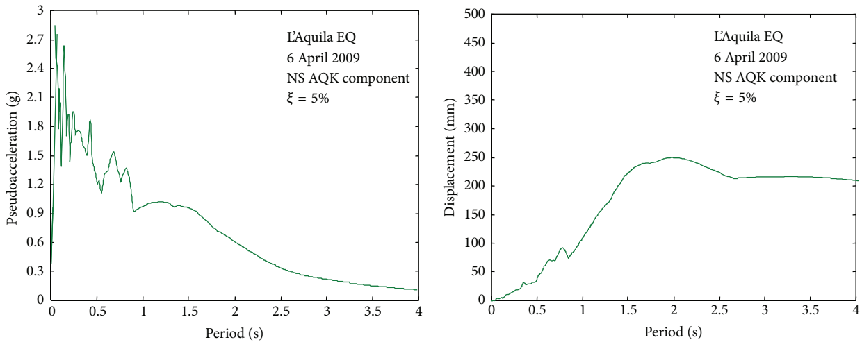
FIGURE 11: Pseudoacceleration and displacement elastic response spectra at \xi = 5\% of NS AQK component—L' Aquila earthquake of 6th of April 2009.
