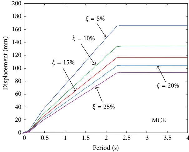
FIGURE 6: Normative displacement elastic response spectrum for Sesto Fiorentino—MCE level, \xi = 5\% , 10\% , 15\% , 20\% , and 25\% , V_n = 50 years, coefficient of use c_u = 1 , topographic category T1, and C-type soil.
