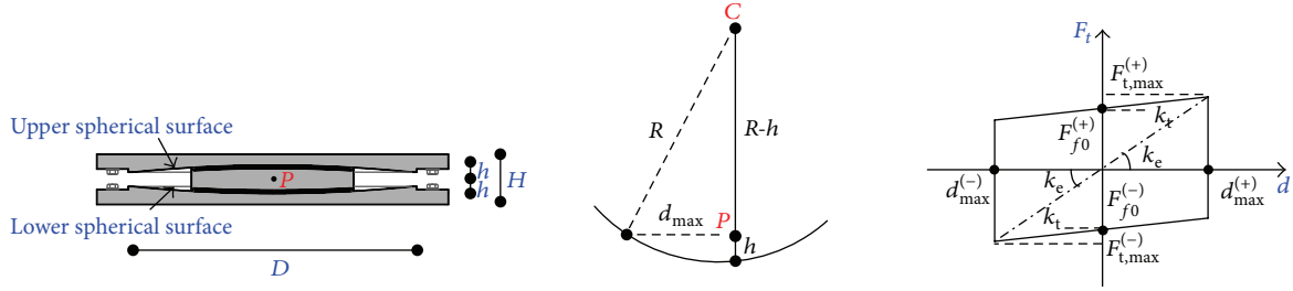
FIGURE 5: Cross section of a symmetrical DFP isolator, characterized by equal concave surfaces and friction coefficients, geometrical parameters of each spherical surface, and corresponding schematic F_t - d response cycle.
