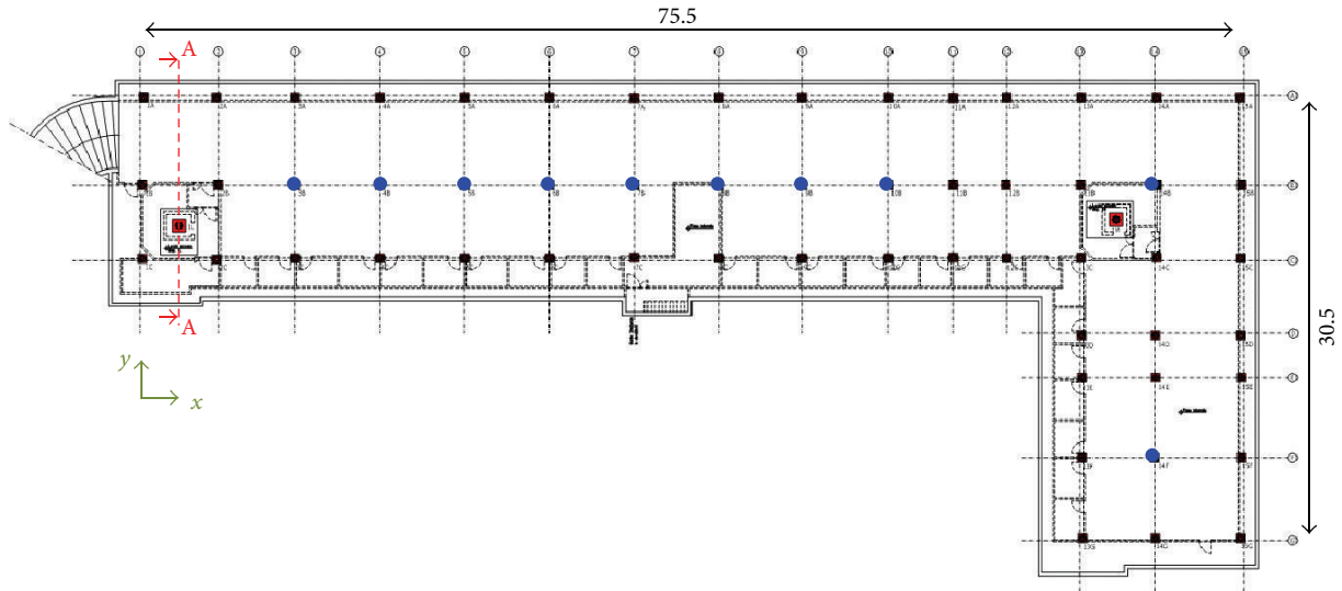
FIGURE 1: Basement plan of the building highlighting the positions of all 59 DFP isolators (squares: A-type; circles: B-type).
