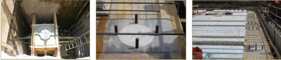
FIGURE 15: Images of the installation works of a DFP isolator placed below the bottom R/C slab of an elevator (left) and some isolators with the top cylindrical caps screwed before casting the relevant upper R/C beam.
