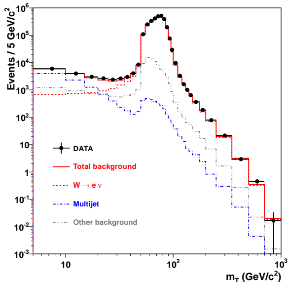
FIG. 2: The transverse mass distributions of e\nu candidate events compared to the total backgrounds.
