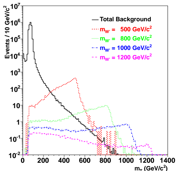
FIG. 1: The transverse mass distributions for W' \rightarrow e\nu signal events generated using PYTHIA with total background expectation.
