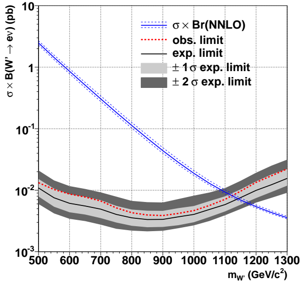
FIG. 3: The 95 % CL limits on cross section times branching fraction as a function of W' boson mass and the expected limits from the simulated experiments with background only. The region above the red dashed line is excluded at the 95 % CL. The cross section times branching fraction assuming the manifest LR symmetric model, \sigma \cdot \mathcal{B}(W' \rightarrow e\nu)_{LR} , is shown along with its uncertainty. The intercept of the cross section limit curve and the lower bound of the theoretical cross section yields m_{W'} > 1.12 \text{ TeV}/c^2 at the 95 % CL.
