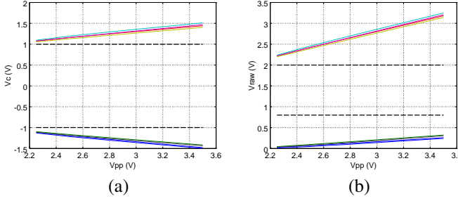
Figure 8. (a) V_{eq} vs. supply voltage for differently unbalanced PUCs. (b) V_{raw} vs. supply voltage.
