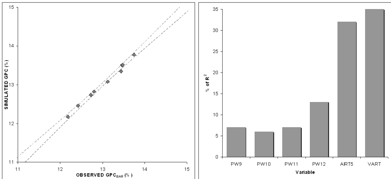
Figure 4a Comparison between Barilla Map Quality surveys for durum wheat grain protein content and simulated grain protein content (TP model) over the four study areas, for a period of 9 years (1999-2007). Statistically significant correlation with an r of 0.99 and p -value= 0.0080. Confidence interval (0.95) grey dashed lines. Figure 4b Relative Importance Metrics for linear model, R^2 partitioned by averaging over orders and normalized to sum 100%
