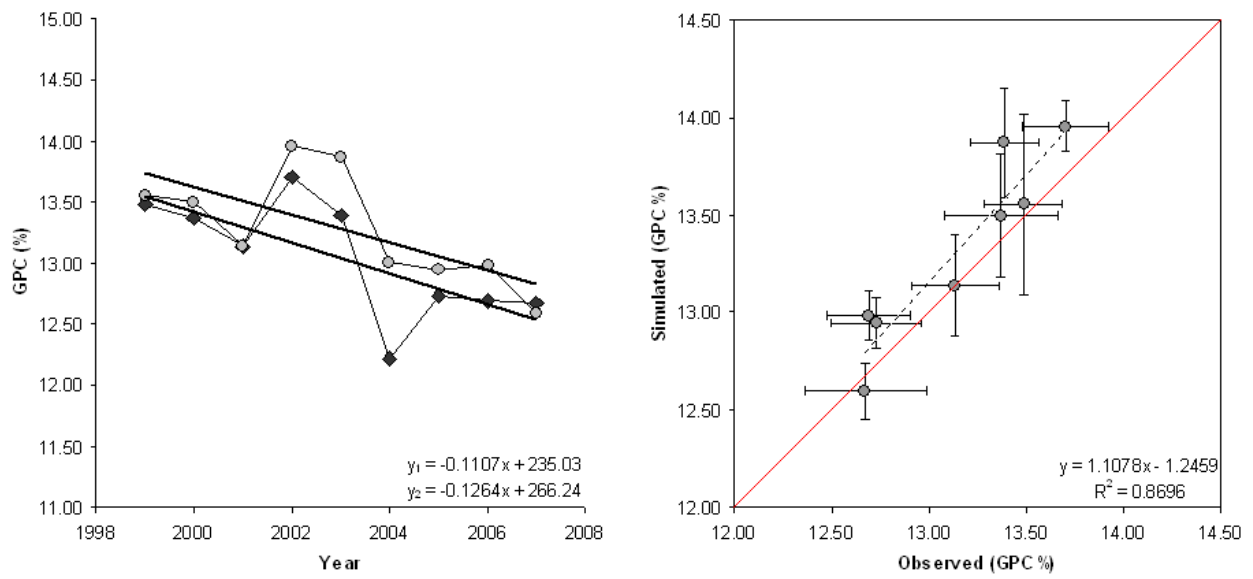
Figure 4a Trend in GPC simulated (Delphi ●, y1) observed (Barilla ♦, y2); Figure 4b Comparison between GPC_{BAR} and GPC_{DEL} over four study areas for the period 1999-2007 aggregating results, excluding 2004. The 1:1 line is shown in figure 4b
