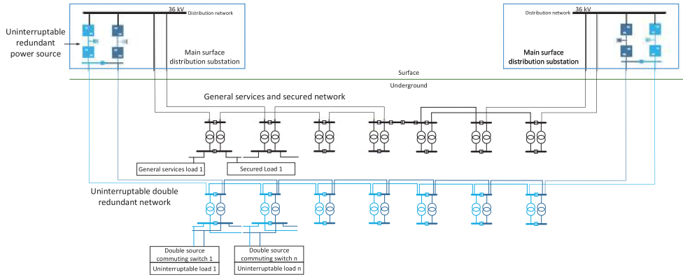
Fig. 5.11. Functional scheme of the general services load network and the doubly redundant uninterruptable load network.
