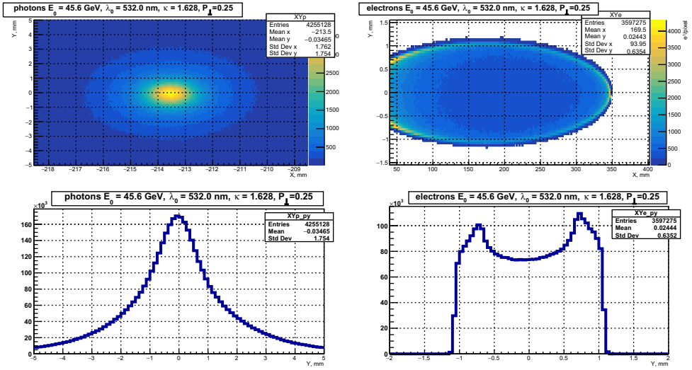
Fig. 3.29. MC results for P_{\perp} = \xi_{\parallel} \zeta_{\perp} = 0.25 and \phi_{\perp} = \pi/2 .
