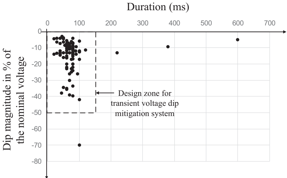
Fig. 5.9. Typical distribution of transient voltage dips recorded within the existing CERN network (collected between 2011 and 2017); the design zone covers most of the transient voltage dips, which are within 0–150 ms and 0–50% magnitude.
