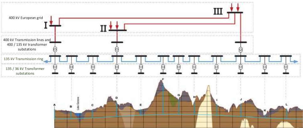
Fig. 5.6. Schematic representation of the transmission network.
