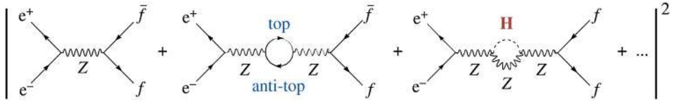
Fig. 1.3. Schematic representation of the perturbative expansion for calculating the cross section for e^+e^- annihilation into a pair of leptons or quarks (denoted f , for fermions); the representative higher order diagrams involving quantum loops with a top quark or a Higgs boson are indicated.
