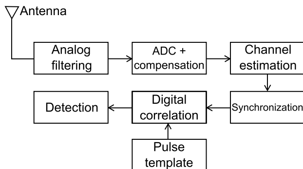
FIGURE 1. Block diagram of the receiver.
