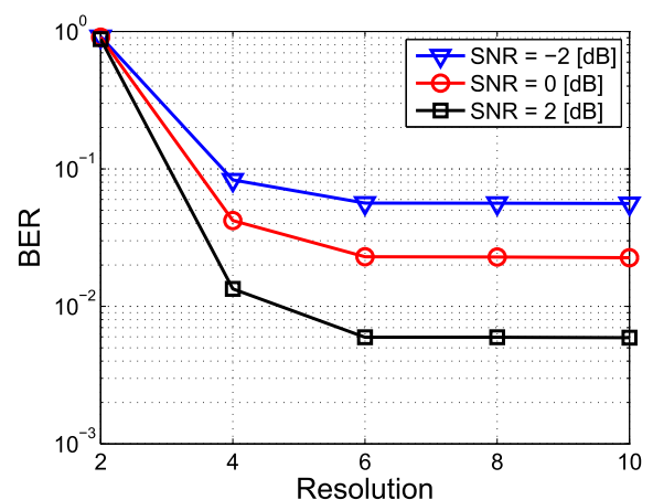
FIGURE 6. BER as a function of ADC resolution for 3 SNR scenarios for an OSR = 2.
