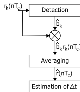
FIGURE 3. Diagram of the estimation process and the signals involved.
