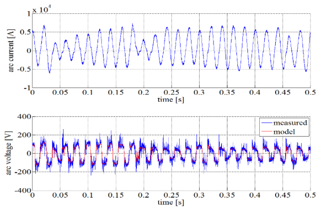
Fig. 9. Measured arc current and voltage.
