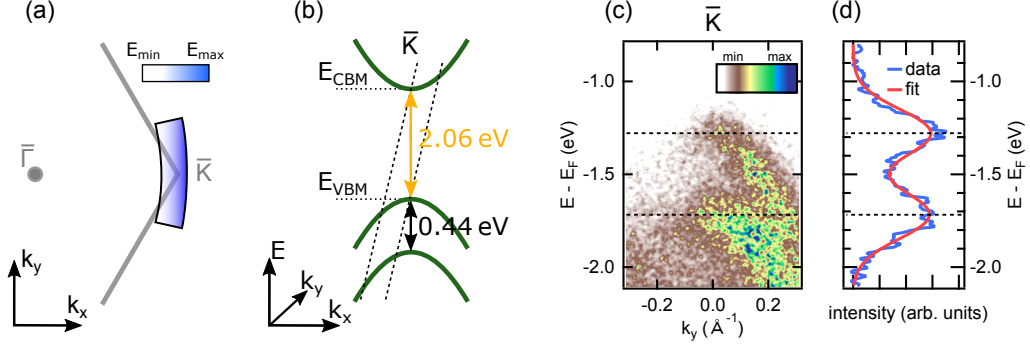
FIG. S1. ARPES data of WS_2/Au(111) taken at \bar{K} for an energy-momentum cut through the VBM. (a) Energy-momentum cut with the analyzer slit oriented perpendicular to the \bar{\Gamma}\bar{K} direction. The color coded area illustrates the relation between k_x and E_{kin} for a cut as investigated in the present study. (b) Schematic illustration of the energy-momentum cuts (dashed lines) through VBM and CBM chosen for the ARPES spectra shown in Fig. 1(b) of the main text and in Fig. S1(c) of the supplemental material, respectively. Note that the band structure is displayed along k_x , which is perpendicular to the entrance slit of the analyzer. (c) ARPES spectrum for an energy-momentum cut through the VBM showing the spin split upper and lower VB. (d) Background subtracted EDC integrated over a momentum window of 0.1 \text{ \AA}^{-1} . The red line shows the result of a fit of two Gaussians to the EDC.
