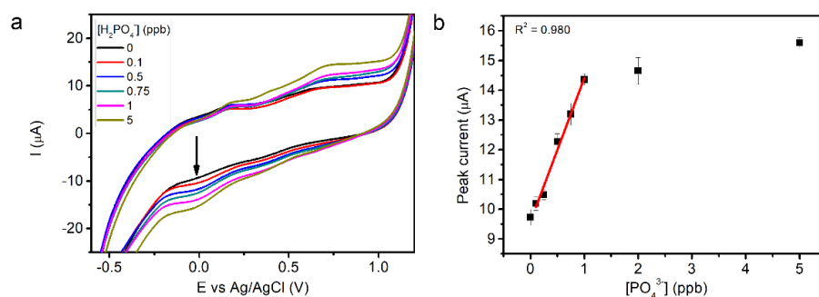
Figure 3 – (a) Cyclic voltammetry performed with different concentrations of phosphate (b) Analytical curve showing the detection range and the lineal range of detection.
