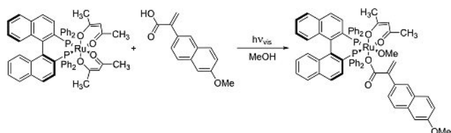
Scheme 1. Light activation of Ru(acac) 2 [(S)-BINAP] for the HY of alkenes.
