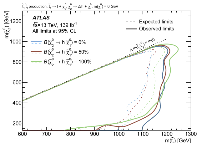
Fig. 11 Exclusion limits at 95% CL on the masses of the \tilde{t}_1 and \tilde{\chi}_2^0 , for a fixed m(\tilde{\chi}_1^0) = 0 GeV and different values of \mathcal{B}(\tilde{\chi}_2^0 \rightarrow h\tilde{\chi}_1^0) with \mathcal{B}(\tilde{\chi}_2^0 \rightarrow Z\tilde{\chi}_1^0) = 1 - \mathcal{B}(\tilde{\chi}_2^0 \rightarrow h\tilde{\chi}_1^0) . The dashed and solid lines are the expected and observed limits for the central value of the signal cross-section, respectively. The expected and observed limits do not include the effect of the theoretical uncertainties in the signal cross-section
