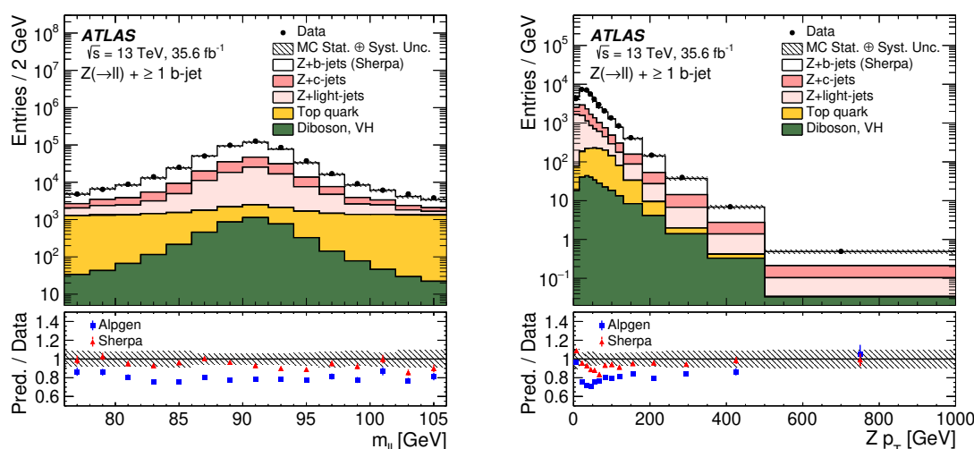
Figure 4. Distribution of events passing the signal selection as a function of m_{\ell\ell} (left) and p_{T,Z} (right) for events with at least one b -jet. The lower panels display the ratio of the predictions for signal plus background to data using either SHERPA (red) or ALPGEN + PYTHIA6 (blue) as the signal simulation. The statistical uncertainty of the data is shown as black error bars and the total uncertainty of the prediction as a hatched band. The latter consists of the statistical uncertainty and all systematic uncertainties from the predictions.
