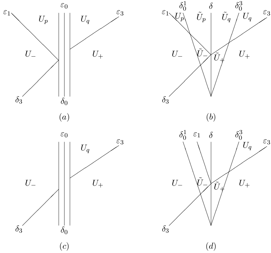
Figure 6: Interaction of a 3-wave \delta_3 with a composite wave \delta_0 . (a), (c): the actual Riemann solvers, the Accurate case (a) and the Simplified one (c); (b), (d): the auxiliary pictures, the Accurate case (b) and the Simplified one (d).
