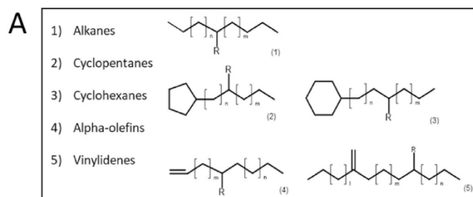
Fig. 2. Structures of MOSH (Left) and MOAH (Right), alkylations and hydrogenations exemplarily.
