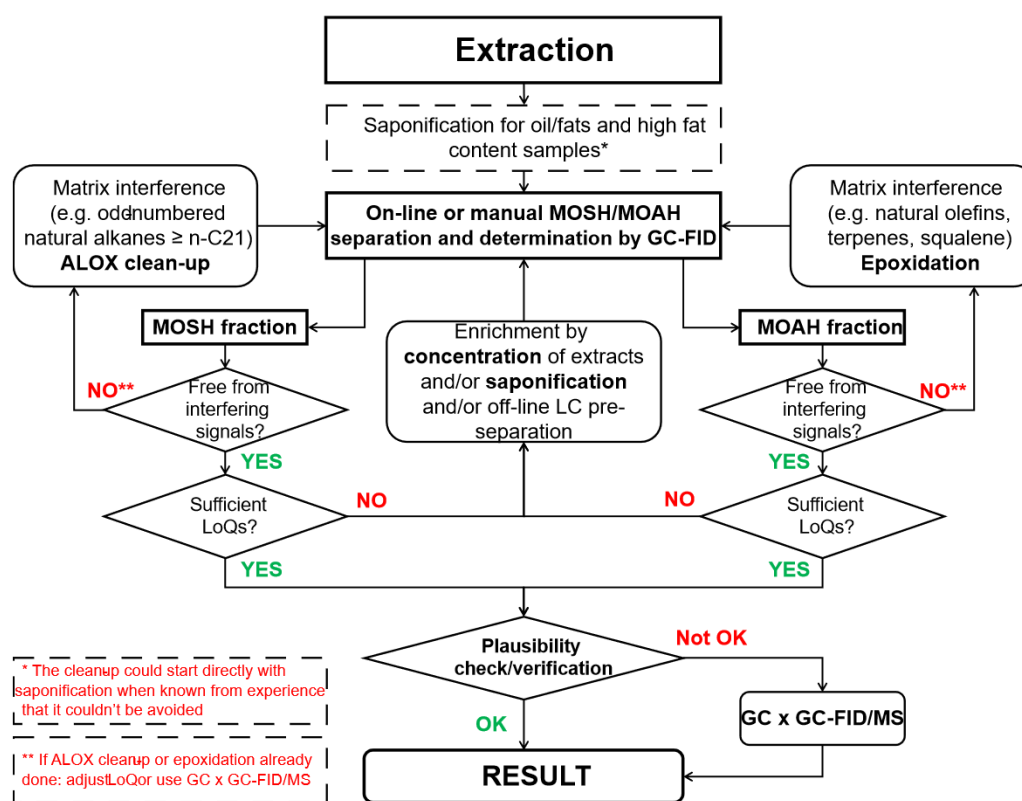
Fig. 4. Decision tree to identify auxiliary methods. Adapted from Bratinova & Hoekstra, 2019. ALOX: Al2O3.
