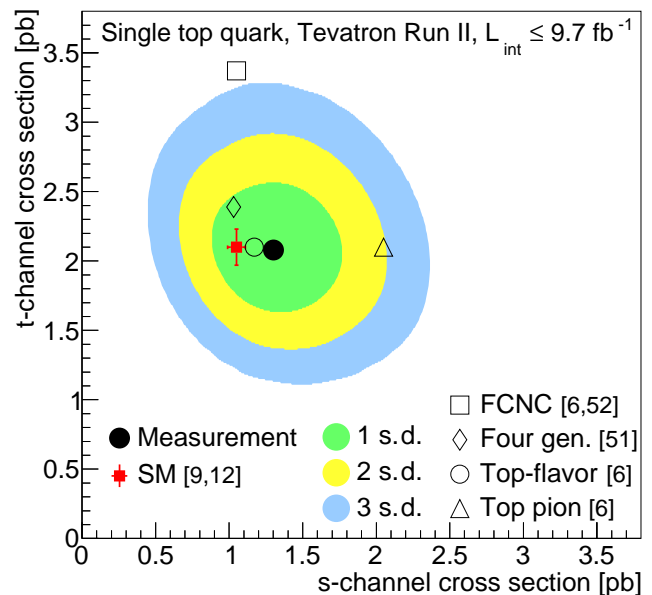
FIG. 2: (Color online) Two-dimensional posterior probability as a function of \sigma_t and \sigma_s with one s. d. (68% C.L.), two s. d. (95% C.L.), and three s. d. (99.7% C.L.) probability contours for the combination of the CDF and D0 analysis channels compared with the NLO+NNLL theoretical prediction of the SM [9, 12]. Several BSM predictions are shown, a model with four quark families with top-to-strange quark coupling |V_{ts}| = 0.2 [54], a top-flavor model with new heavy bosons with mass m_x = 1 TeV [6], a model of charged top-pions with mass m_{\pi^\pm} = 250 GeV [6], and a model with flavor-changing neutral currents with a 0.036 coupling \kappa_u/\Lambda between up quark, top quark and gluon [6, 55].
