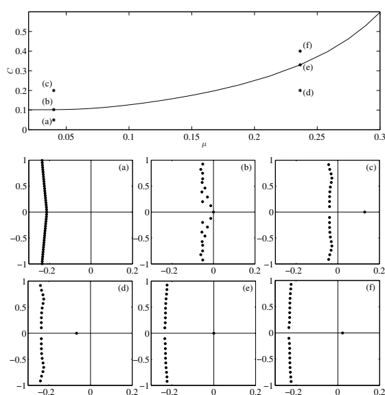
FIG. 3. Existence boundary in the (\mu, C) -parameter plane (top panel); eigenvalues of the trivial equilibrium corresponding to points * in the top panel (panels (a)–(f)): relevant parameter values at machine precision are \mu = 0.040030019682702 (a)–(c) and 0.236338384280189 (d)–(f) and C = 0.05 (a), 0.102409511357698 (b), 0.2 (c)–(d), 0.330235018740724 (e), and 0.4 (f).
