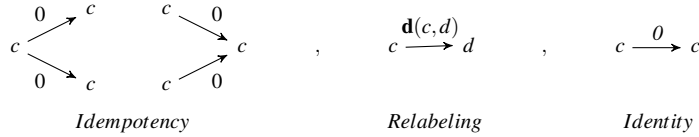
Figure 2: Arcs of the graph representing the transformation of single level trees.
