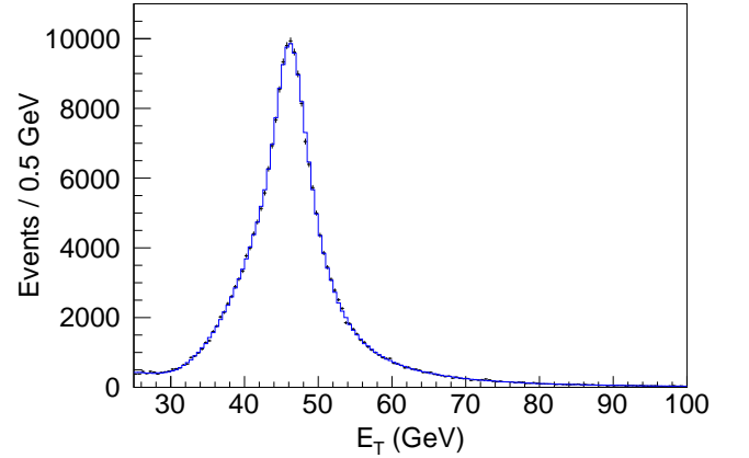
FIG. 14. E_T distribution for the CC-topology electron with the larger E_T . The crosses are the background-subtracted data and the solid histogram is the simulation.
