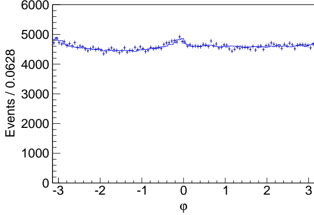
FIG. 11. Distribution of \varphi in the Collins-Soper frame for CC- and CP-topology dielectrons with 66 < M < 116 \text{ GeV}/c^2 . The crosses are the background-subtracted data and the solid histogram is the simulation.
