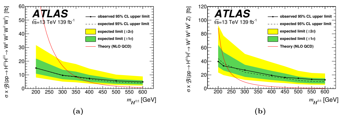
Figure 9. Observed and expected upper limits on the (a) H^{\pm\pm} pair production and (b) H^{\pm\pm} and H^\pm associated production cross section times branching fraction at 95% CL obtained from the combination of 2\ell^{sc} , 3\ell and 4\ell channels. The region above the observed limit is excluded by the measurement. The bands represent the expected exclusion curves within one and two standard deviations. The theoretical prediction [29] including the NLO QCD corrections [52] is also shown.
