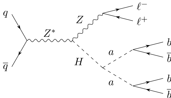
Figure 1. Tree-level Feynman diagram representing ZH production with H \rightarrow aa \rightarrow \bar{b}b\bar{b} .
