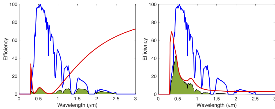
Fig. 4. Similar to Fig. 3, the figure shows examples of the results used to optimize the periodically loaded surface of Fig. 1. In both the panels, the blue curve is the solar PSD [44]. The red curve is the percentage of power that is reflected (left panel) or dissipated (right panel) by antennas in the lattice. The product between these two curves delimits the green-filled region. The ratio between the areas of the green-filled region, and the region below the blue curve gives the total percentage of power that is reflected (left panel) or absorbed (right panel).
