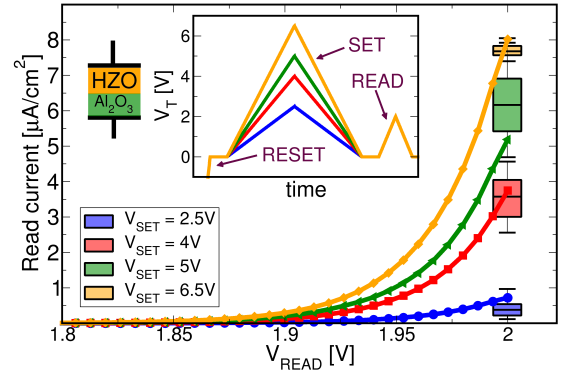
Fig. 5: Simulations for the read current of an HZO/ \text{Al}_2\text{O}_3 FTJ ( t_F = 12\text{nm} , t_D = 2\text{nm} ) versus read voltage V_R . The box plots for experiments were inferred from the cycle to cycle variations reported Fig.3(d) of [29] (device area \approx 3.14 \cdot 10^{-4} \text{ cm}^2 ). The inset shows the signal waveforms for the write and read operation. The reset voltage is -8\text{V} .
