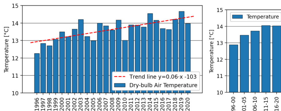
Figure 1. Dry-bulb air temperature annual mean values with trend line and 5-year mean values used in the study.
