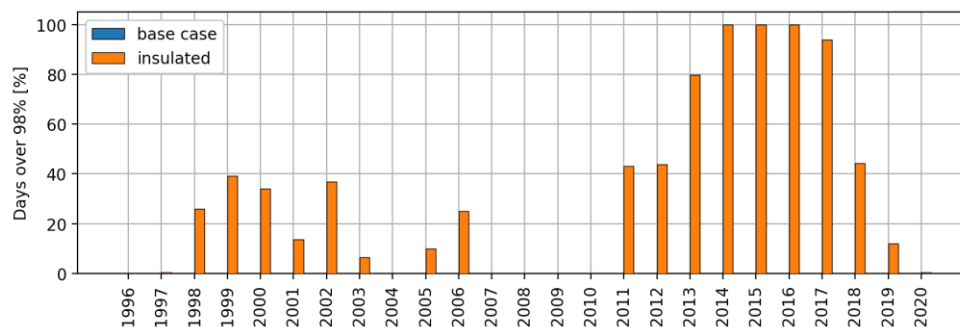
Figure 9. Percentage of days with relative humidity above 98 % RH on the surface of the brick layer facing the insulation for multiyear simulation divided by year.
