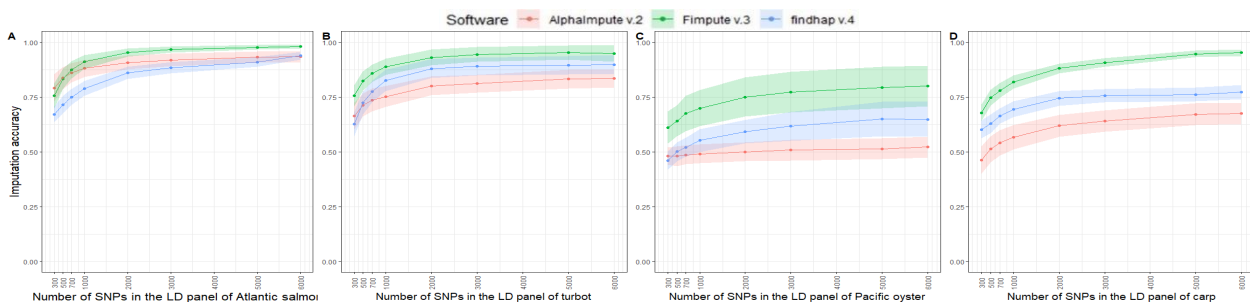
Figure 1. Comparison of genotype imputation accuracy between the three imputation software for Atlantic salmon, turbot, Pacific oyster and carp when selecting SNPs for the LD panel with method 1.
