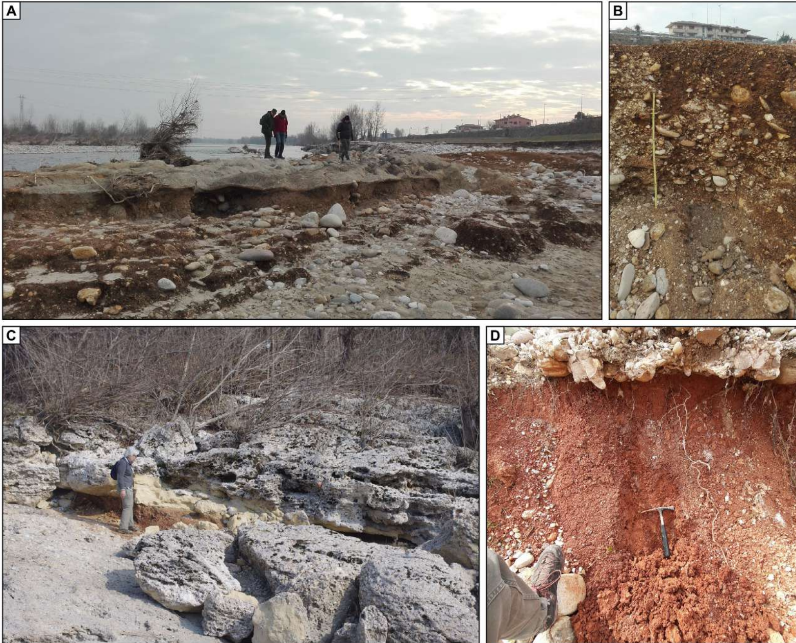
Fig. 7 - Photos of the outcrops related to Stop 1.1. A) the palaeosil cropping out in the western side of Piave thalweg at Nervesa; B) detail of the palaeosil; C) Early Pleistocene conglomerates cropping out along the Piave thalweg; D) the palaeosil cropping out in the eastern side of the Piave section at Nervesa.
