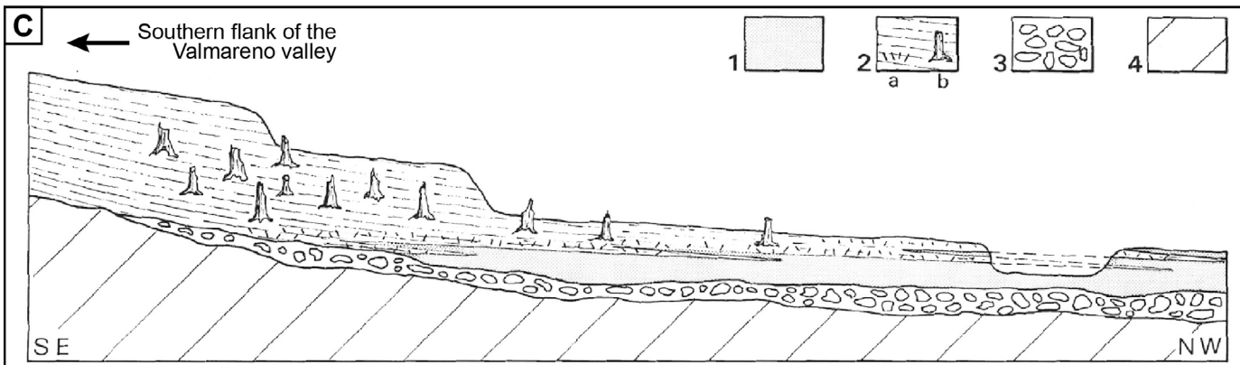
Fig. 12 - A) Photo of the lacustrine deposits of Revine embedding larch trunks in life position (Stop 1.3); B) Detail of the laminated lacustrine deposits; C) Geological sketch of the Revine succession cropping out in the clay pit; legend: 1) Lacustrine deposits; 2) Slope deposits with roots and larch logs in place; 3) Glacial and glaciofluvial deposits, 4) Bedrock (photos and scheme from Casadoro et al., 1976).
