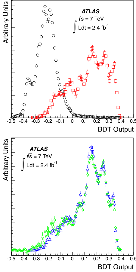
Fig. 5. Distributions of the response of the BDT classifier. Top: B_s^0 \rightarrow \mu^+\mu^- MC sample (squares) and data sidebands (circles); bottom: B \rightarrow J/\psi K events from tuned MC samples (triangles) and sideband-subtracted data (stars).
