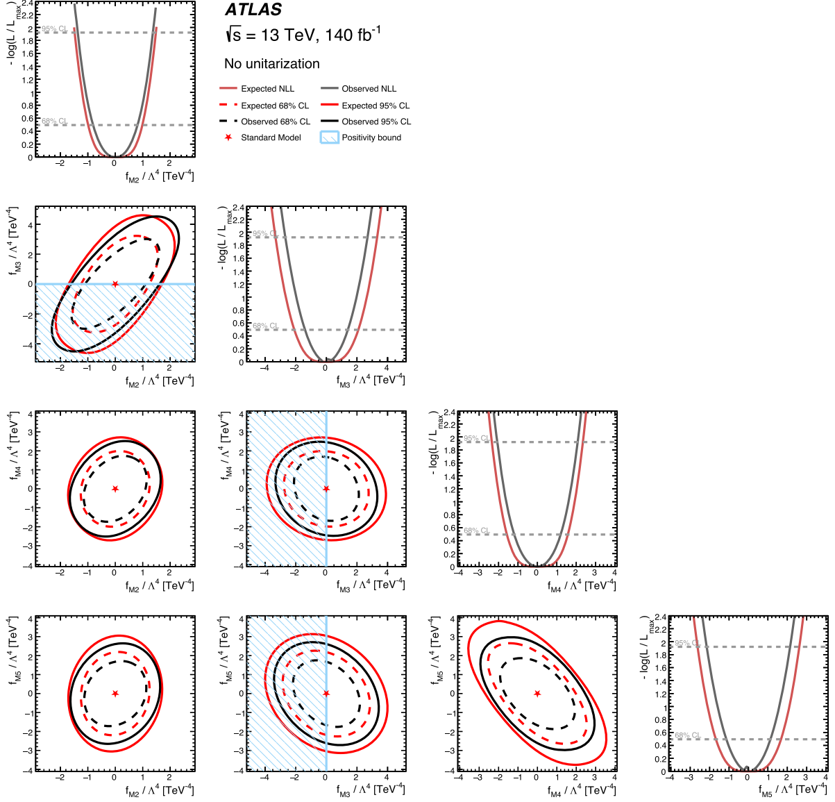
Fig. 5. Expected (red) and observed (black) 68% (dashed) and 95% (solid) confidence level contours when considering two of the f_{M2} , f_{M3} , f_{M4} , and f_{M5} coefficients simultaneously alongside the relevant cross-term. The expected (greyed-red) and observed (grey) negative log-likelihood (NLL) curve for each of the operators when considering just one coefficient at a time is also shown. Unitarity constraints are not visible and positivity bounds are overlaid as a blue filled region.
