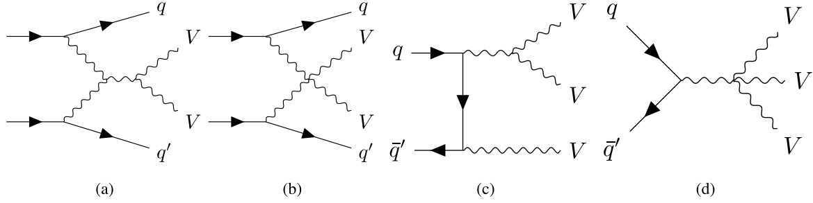
Fig. 1. Representative Feynman diagrams for a) vector-boson scattering with triple-gauge vertices, b) vector-boson scattering with quartic-gauge vertices, c) tri-boson production with triple-gauge vertices, and d) tri-boson production with quartic-gauge vertices. The aQGCs act only on diagrams b) and d) through anomalous values or vertices forbidden in the SM.
