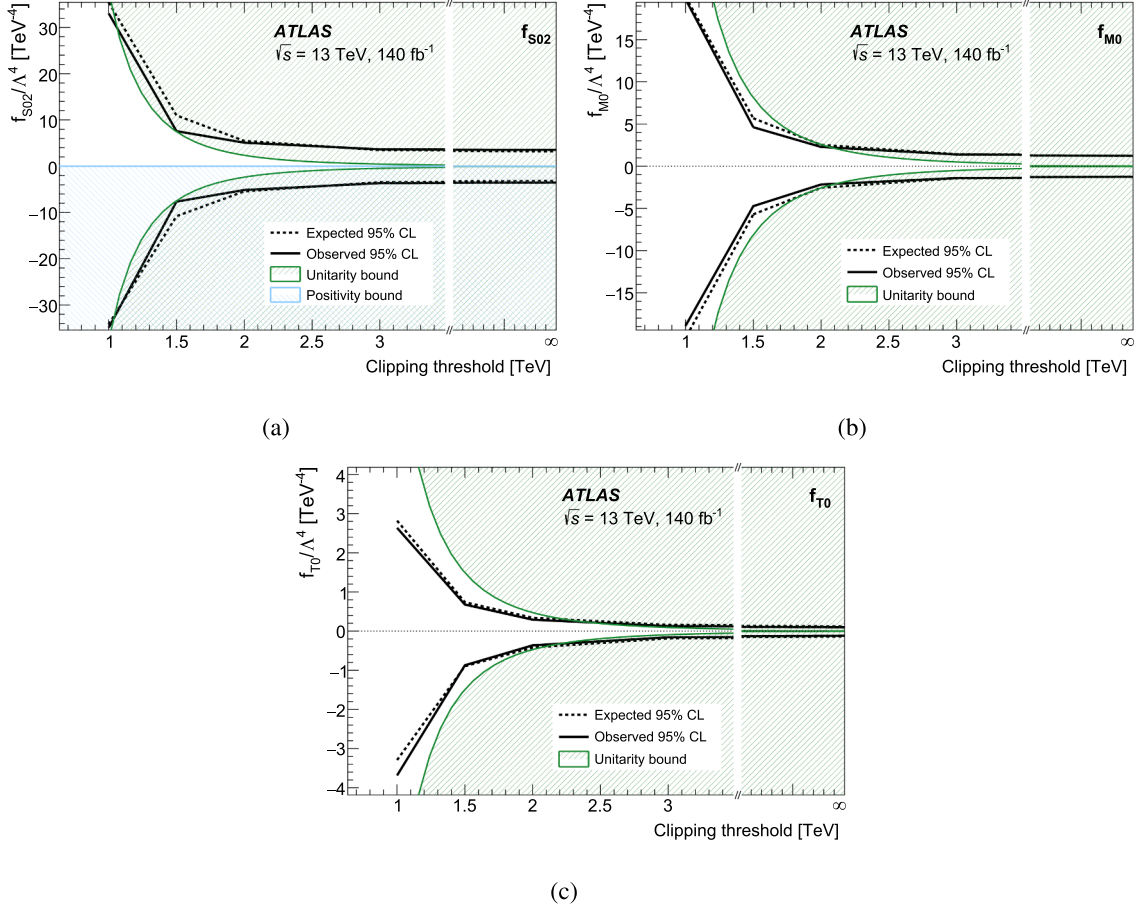
Fig. 4. Expected and observed 95% confidence level confidence intervals on the a) f_{S02} , b) f_{M0} and c) f_{T0} Wilson coefficients as a function of clipping threshold. Unitarity and positivity bounds are shown in green and blue respectively. Unitarized intervals are taken to be the intersection between the interpolated confidence intervals and the unitarity bound.
