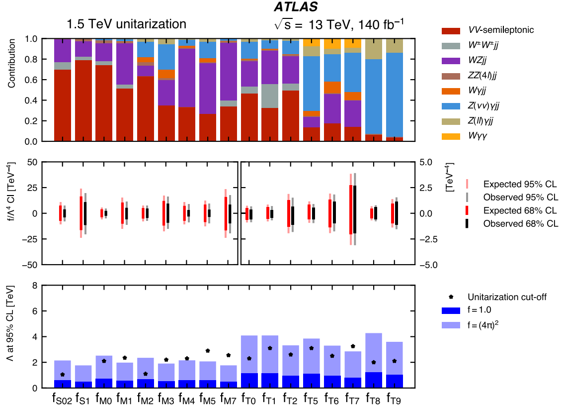
Fig. 3. Contributions of the individual channels to the combination (top), expected and observed 68% and 95% confidence level intervals from the combined fit (middle) and the probed energy scale for two illustrative values of the Wilson coefficients (bottom). Unitarity is preserved by setting higher dimension operator contributions to zero above a clipping threshold of 1.5 TeV. The energy scale of the observed unitarization cut-off as evaluated through a clipping procedure is overlaid on the bottom panel. No unitarization cut-off is found for the f_{S1} coefficient where the experimental interval is always weaker than the unitarity constraint.
