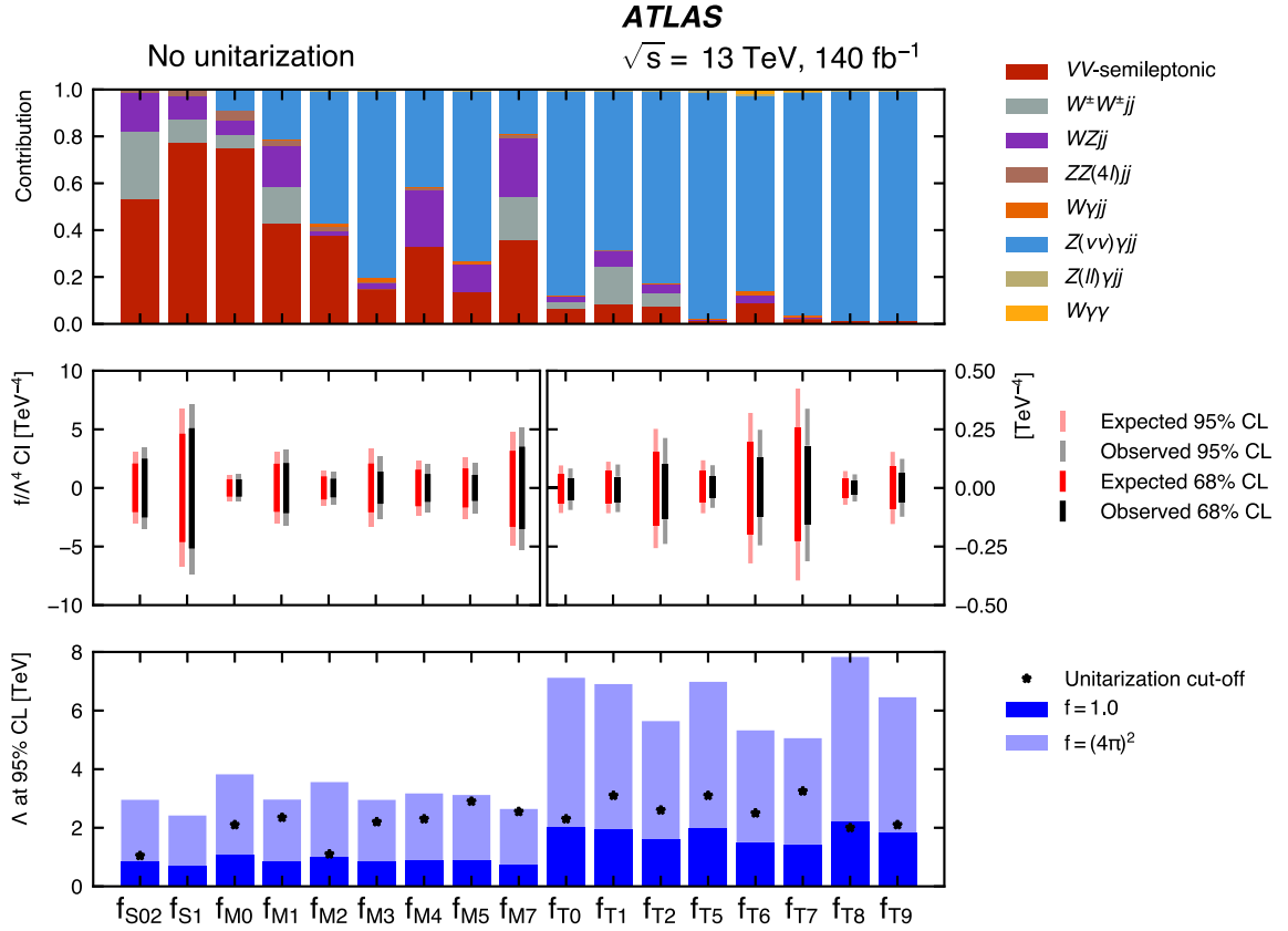
Fig. 2. Contributions of the individual channels to the combination (top), expected and observed 68% and 95% confidence level intervals from the combined fit (middle) and the probed energy scale for two illustrative values of the Wilson coefficients (bottom). No constraints from unitarity bounds are applied. The energy scale of the observed unitarization cut-off as evaluated through a clipping procedure is overlaid on the bottom panel. No unitarization cut-off is found for the f_{S1} operator where the experimental interval is always weaker than the unitarity constraint.
