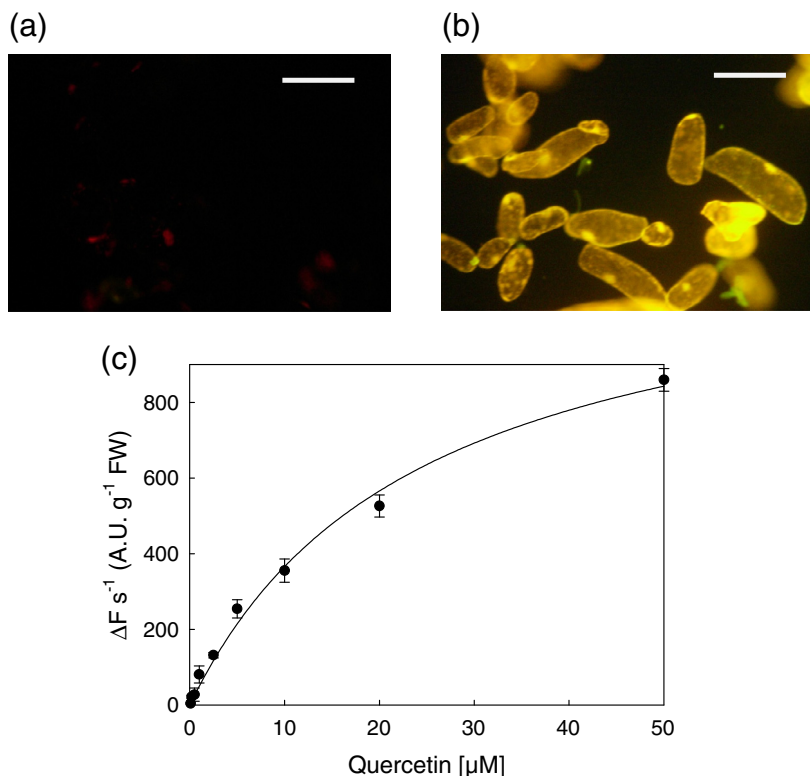
Fig. 2. Panels (a) and (b): images under fluorescent light of grapevine NPC treated either with DPBA (a) or with both DPBA and QC (b). Scale bars = 50 μm. Panel (c): in vivo QC uptake in grapevine suspension cell cultures, measured by means of DPBA fluorescence. Values represent a mean of five independent replicates ± SD. Regression curve (single rectangular hyperbola) was obtained using the following equation: y = a \cdot x / (b + x) ; a = 1250 \pm 87 \Delta F s^{-1} and b = 24.2 \pm 3.5 \mu M .
