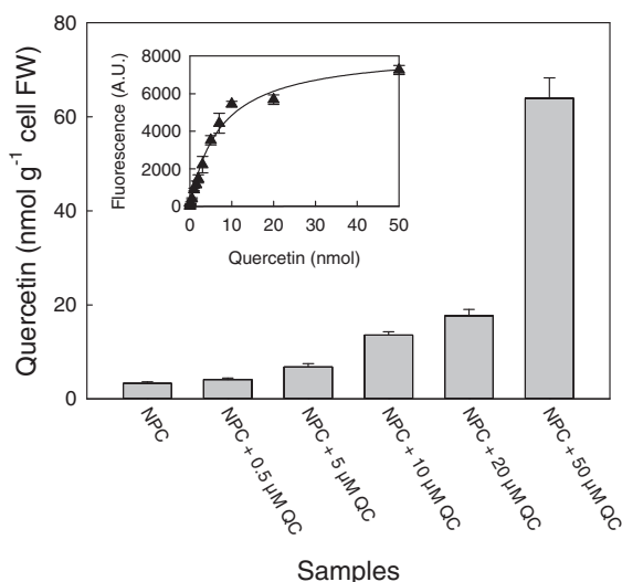
Fig. 5. QC determination in cell methanolic extracts. Different QC concentrations (0.5, 5, 10, 20 and 50 μM, respectively) were added to grapevine suspension cell cultures. The inset plot shows the calibration curve of fluorescence intensity obtained with different amount of QC, ranging from 0 to 50 nmol. Values are means of three independent replicates ± SD.
