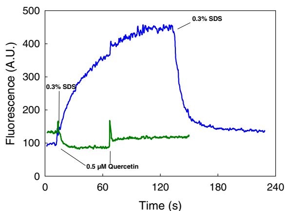
Fig. 3. Spectrofluorimetric analysis of DPBA/QC movement in grapevine suspension cell cultures. Traces are representative of at least three independent replicates. Sonicated cells were used to check DPBA/QC movement within the vesicles, by firstly adding 0.5 μM QC (blue line) or 0.3% SDS (green line), respectively.
