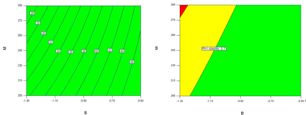
Figure 5 – Equilibrium maps for the RSI_{\min} (left) and Type-I stability (right) for a lateral shredder (with: L=0.2 m, H=0.28 m, \alpha=45^\circ , R=2 m) drawn with respect to the distance B of the implement's CoG to tractor's longitudinal axis ( x axis) and with respect to the mass M ( y axis); different contours have been plotted in the RSI_{\min} equilibrium map to evidence how the index increases (from top-left to down-right)
