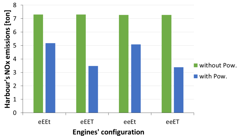
Fig. 7. Annual average NO x harbor emissions for hybrid engine configurations with only one GT, with and without Power management.
