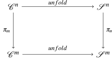
Figure 1: Relating projections of sequences
